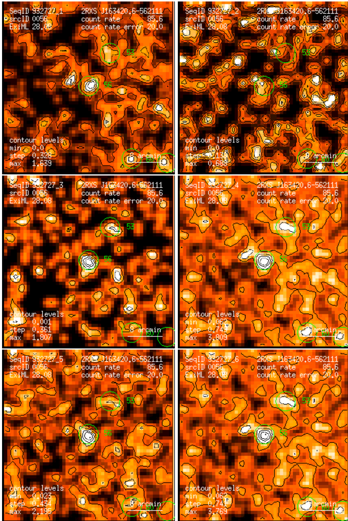
Figure 56: RASS 932727: detection 0056: band rate images, Gaussian filter: (1) PSPC channels 11 – 41, (2) 52 – 90, (3) 91 – 201, (4) 11 – 235, (5) 52 – 201, (6) 11 – 201. Broad band rates in counts/ks. Band rate contour levels in counts/ks/arcmin 2 .
