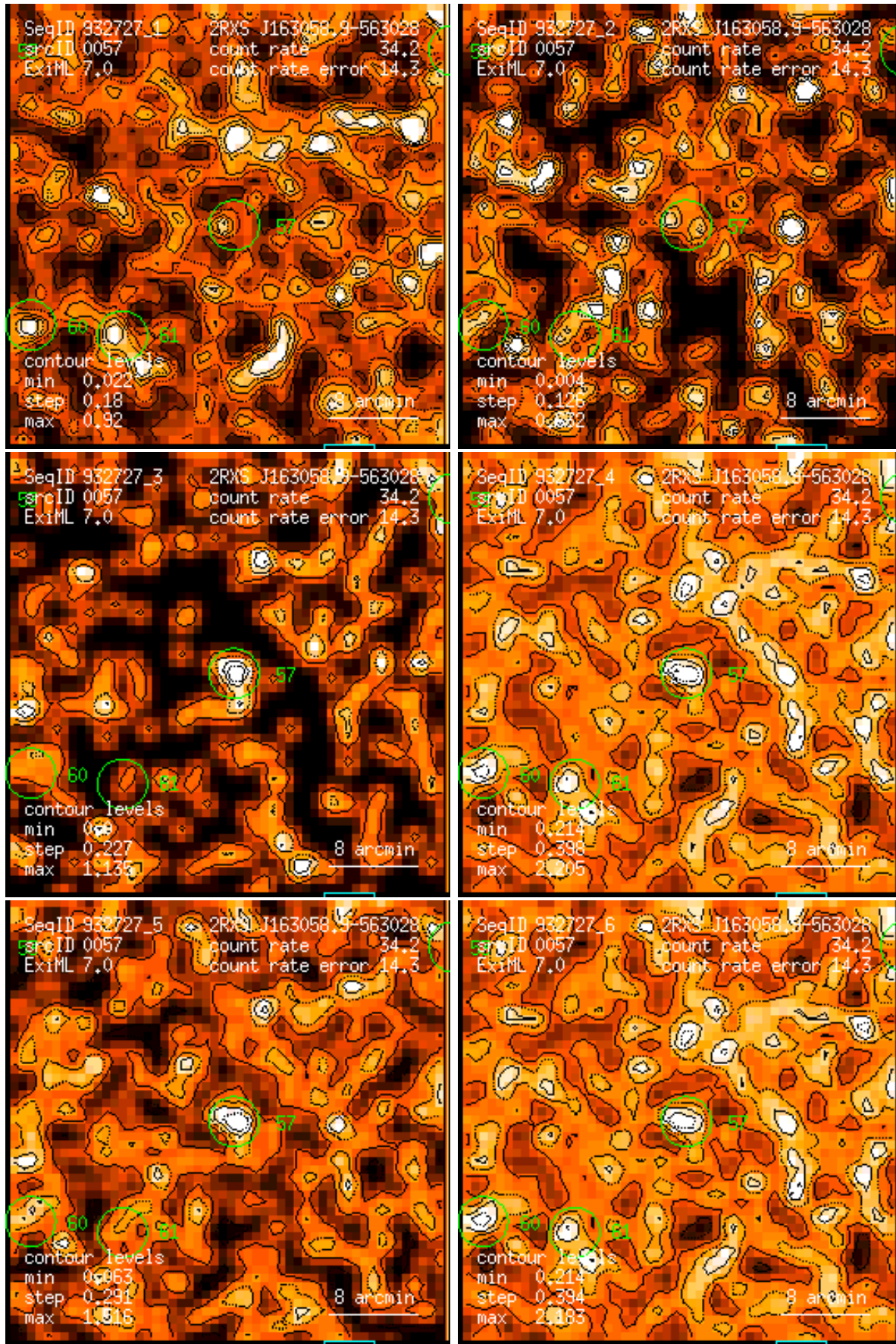
Figure 57: RASS 932727: detection 0057: band rate images, Gaussian filter: (1) PSPC channels 11 – 41, (2) 52 – 90, (3) 91 – 201, (4) 11 – 235, (5) 52 – 201, (6) 11 – 201. Broad band rates in counts/ks. Band rate contour levels in counts/ks/arcmin 2 .
