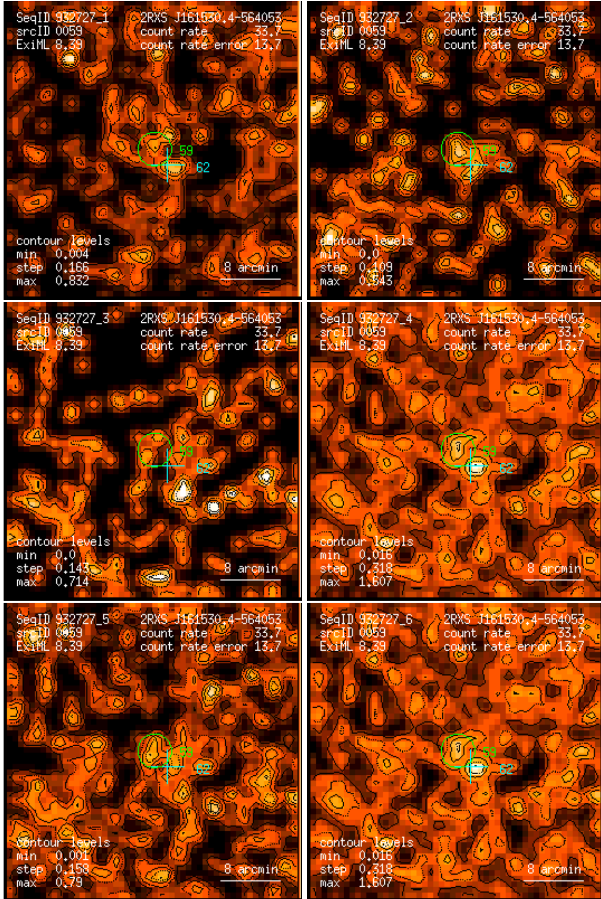
Figure 59: RASS 932727: detection 0059: band rate images, Gaussian filter: (1) PSPC channels 11 – 41, (2) 52 – 90, (3) 91 – 201, (4) 11 – 235, (5) 52 – 201, (6) 11 – 201. Broad band rates in counts/ks. Band rate contour levels in counts/ks/arcmin 2 .
