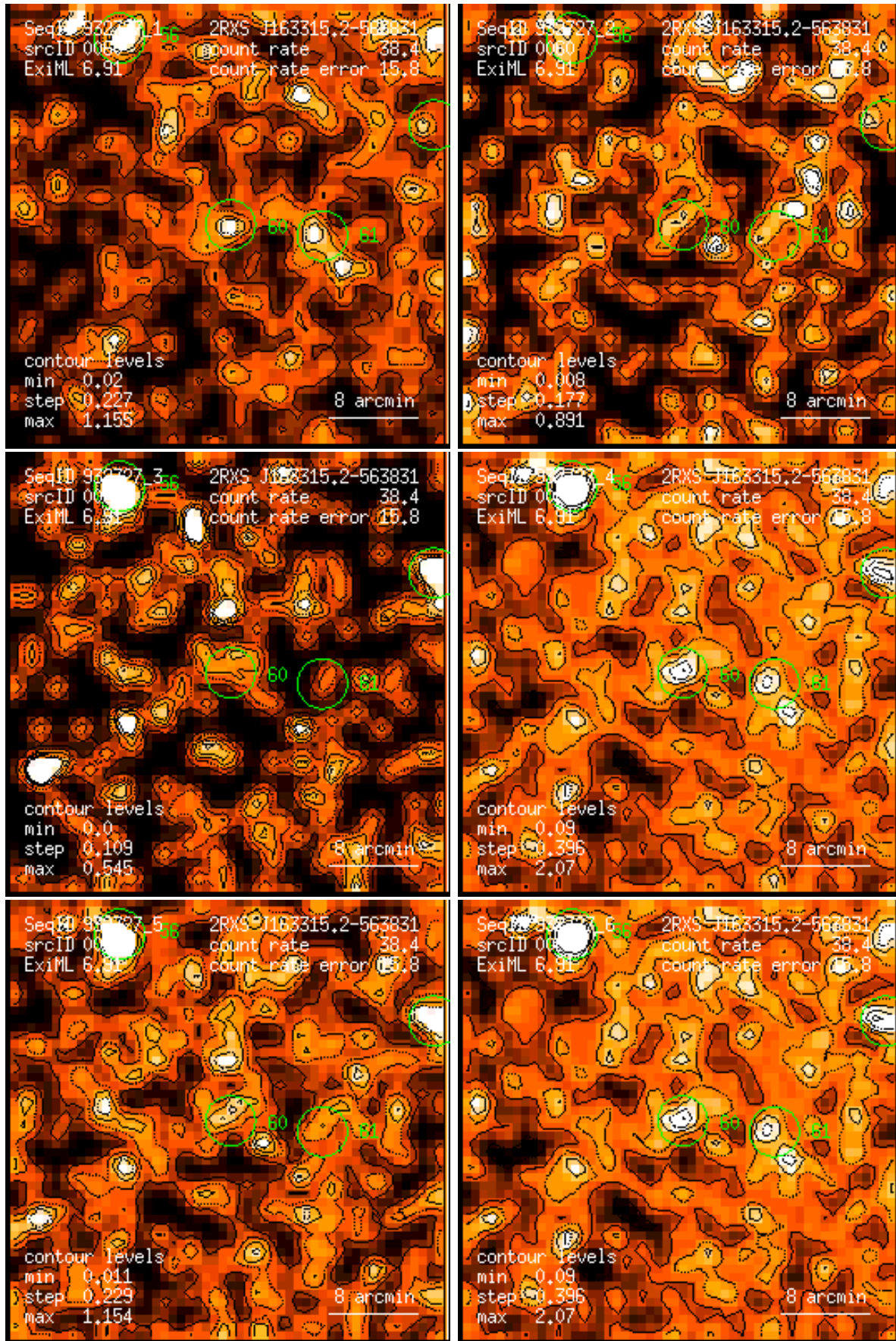
Figure 60: RASS 932727: detection 0060: band rate images, Gaussian filter: (1) PSPC channels 11 – 41, (2) 52 – 90, (3) 91 – 201, (4) 11 – 235, (5) 52 – 201, (6) 11 – 201. Broad band rates in counts/ks. Band rate contour levels in counts/ks/arcmin 2 .
