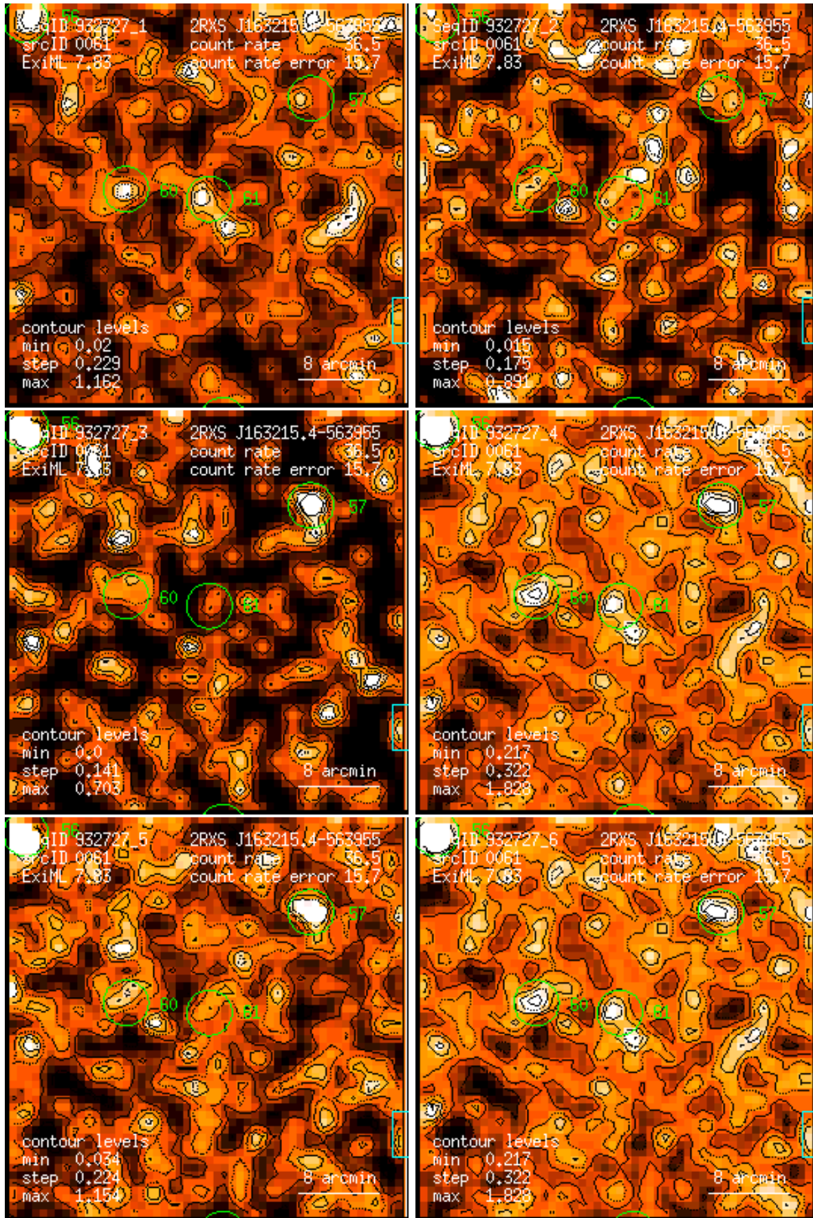
Figure 61: RASS 932727: detection 0061: band rate images, Gaussian filter: (1) PSPC channels 11 – 41, (2) 52 – 90, (3) 91 – 201, (4) 11 – 235, (5) 52 – 201, (6) 11 – 201. Broad band rates in counts/ks. Band rate contour levels in counts/ks/arcmin 2 .
