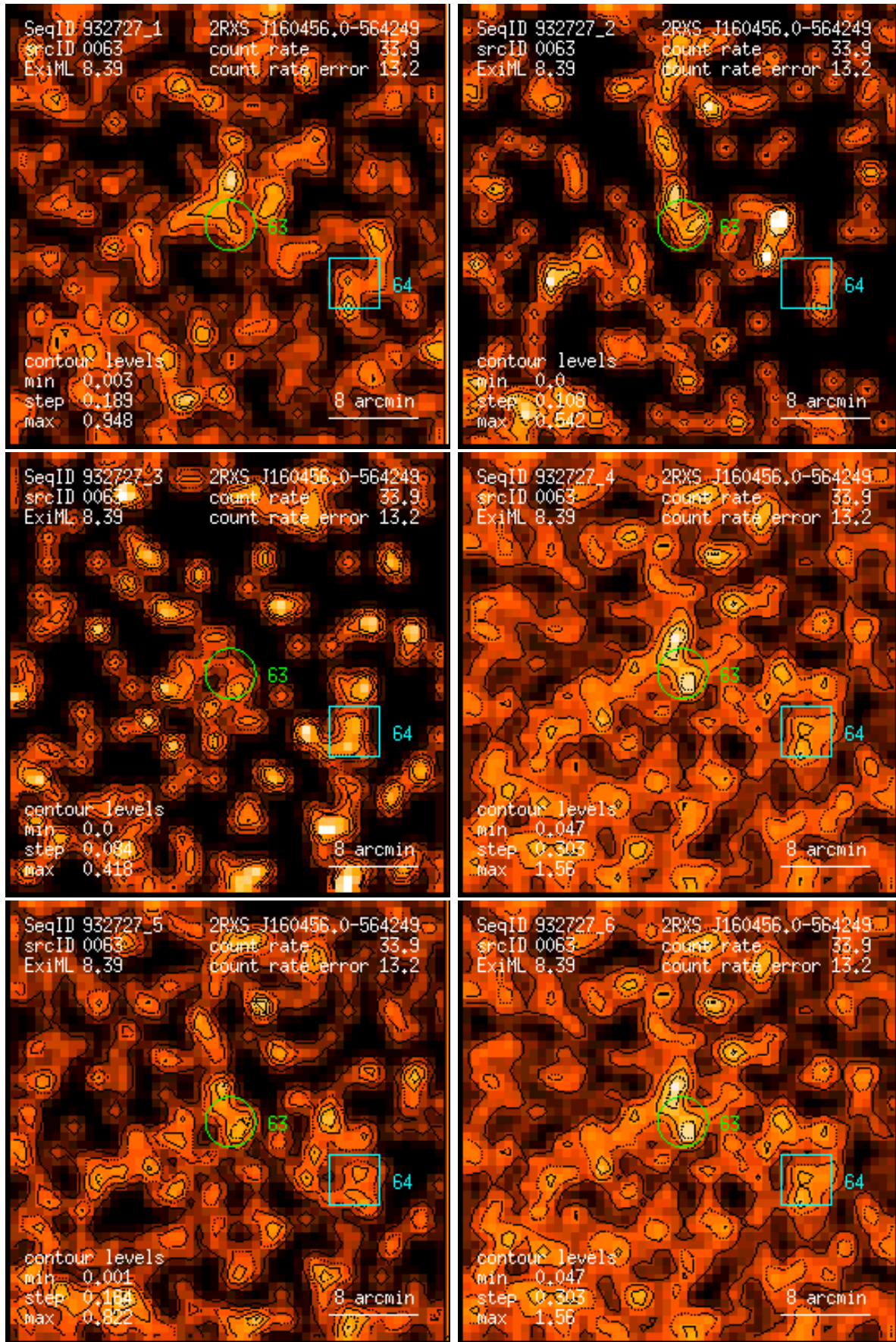
Figure 63: RASS 932727: detection 0063: band rate images, Gaussian filter: (1) PSPC channels 11 – 41, (2) 52 – 90, (3) 91 – 201, (4) 11 – 235, (5) 52 – 201, (6) 11 – 201. Broad band rates in counts/ks. Band rate contour levels in counts/ks/arcmin 2 .
