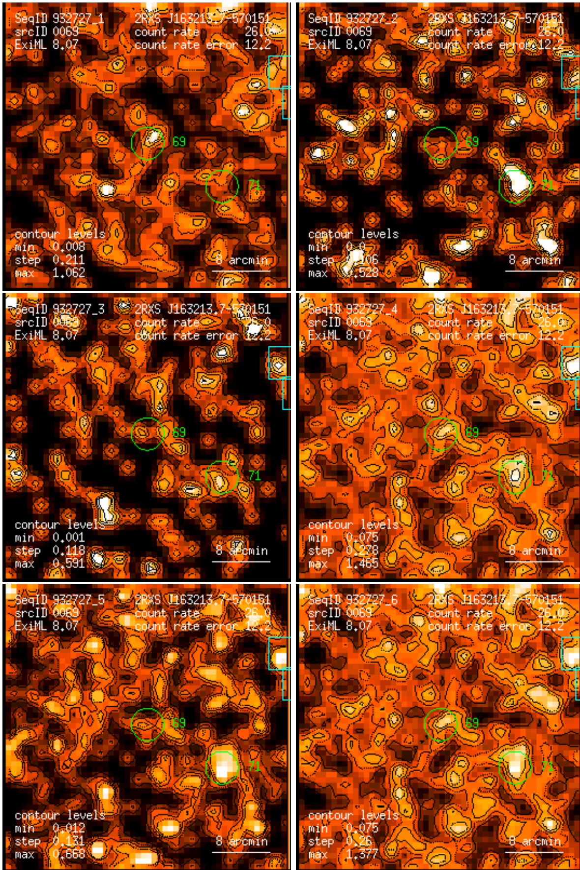
Figure 69: RASS 932727: detection 0069: band rate images, Gaussian filter: (1) PSPC channels 11 – 41, (2) 52 – 90, (3) 91 – 201, (4) 11 – 235, (5) 52 – 201, (6) 11 – 201. Broad band rates in counts/ks. Band rate contour levels in counts/ks/arcmin 2 .
