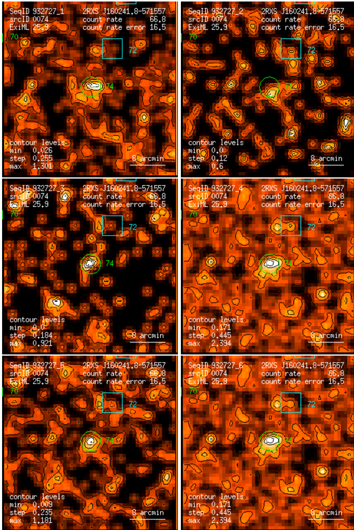
Figure 74: RASS 932727: detection 0074: band rate images, Gaussian filter: (1) PSPC channels 11 – 41, (2) 52 – 90, (3) 91 – 201, (4) 11 – 235, (5) 52 – 201, (6) 11 – 201. Broad band rates in counts/ks. Band rate contour levels in counts/ks/arcmin 2 .
