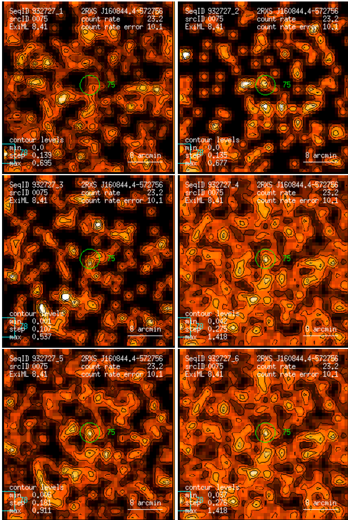
Figure 75: RASS 932727: detection 0075: band rate images, Gaussian filter: (1) PSPC channels 11 – 41, (2) 52 – 90, (3) 91 – 201, (4) 11 – 235, (5) 52 – 201, (6) 11 – 201. Broad band rates in counts/ks. Band rate contour levels in counts/ks/arcmin 2 .
