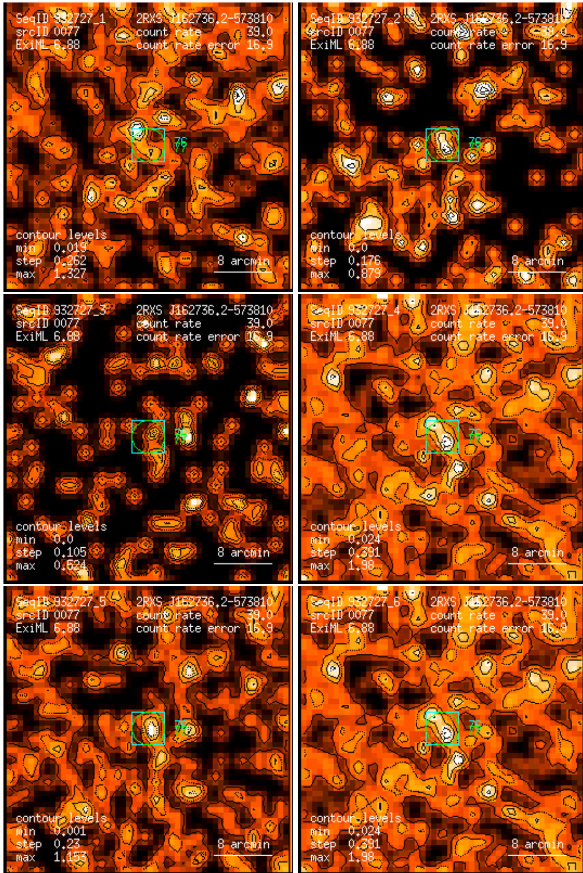
Figure 77: RASS 932727: detection 0077: band rate images, Gaussian filter: (1) PSPC channels 11 – 41, (2) 52 – 90, (3) 91 – 201, (4) 11 – 235, (5) 52 – 201, (6) 11 – 201. Broad band rates in counts/ks. Band rate contour levels in counts/ks/arcmin 2 .
