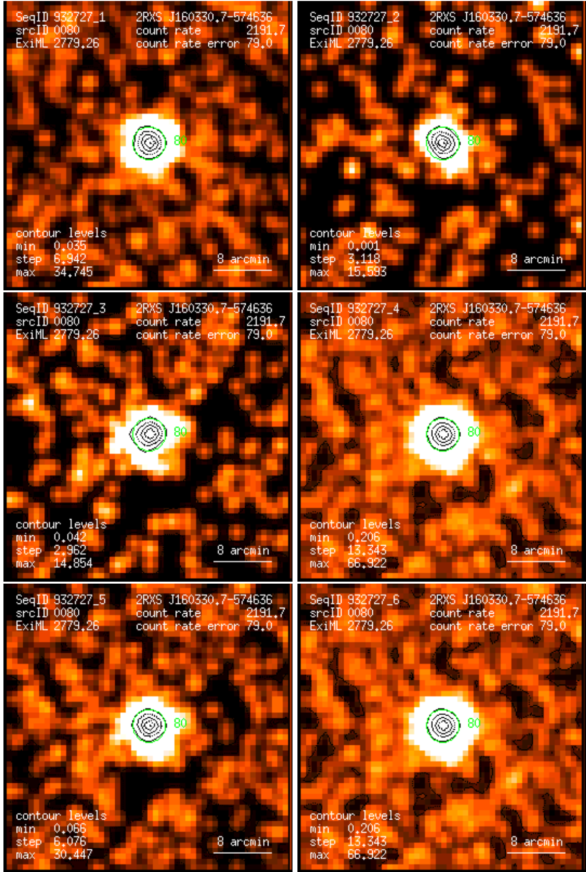
Figure 80: RASS 932727: detection 0080: band rate images, Gaussian filter: (1) PSPC channels 11 – 41, (2) 52 – 90, (3) 91 – 201, (4) 11 – 235, (5) 52 – 201, (6) 11 – 201. Broad band rates in counts/ks. Band rate contour levels in counts/ks/arcmin 2 .
