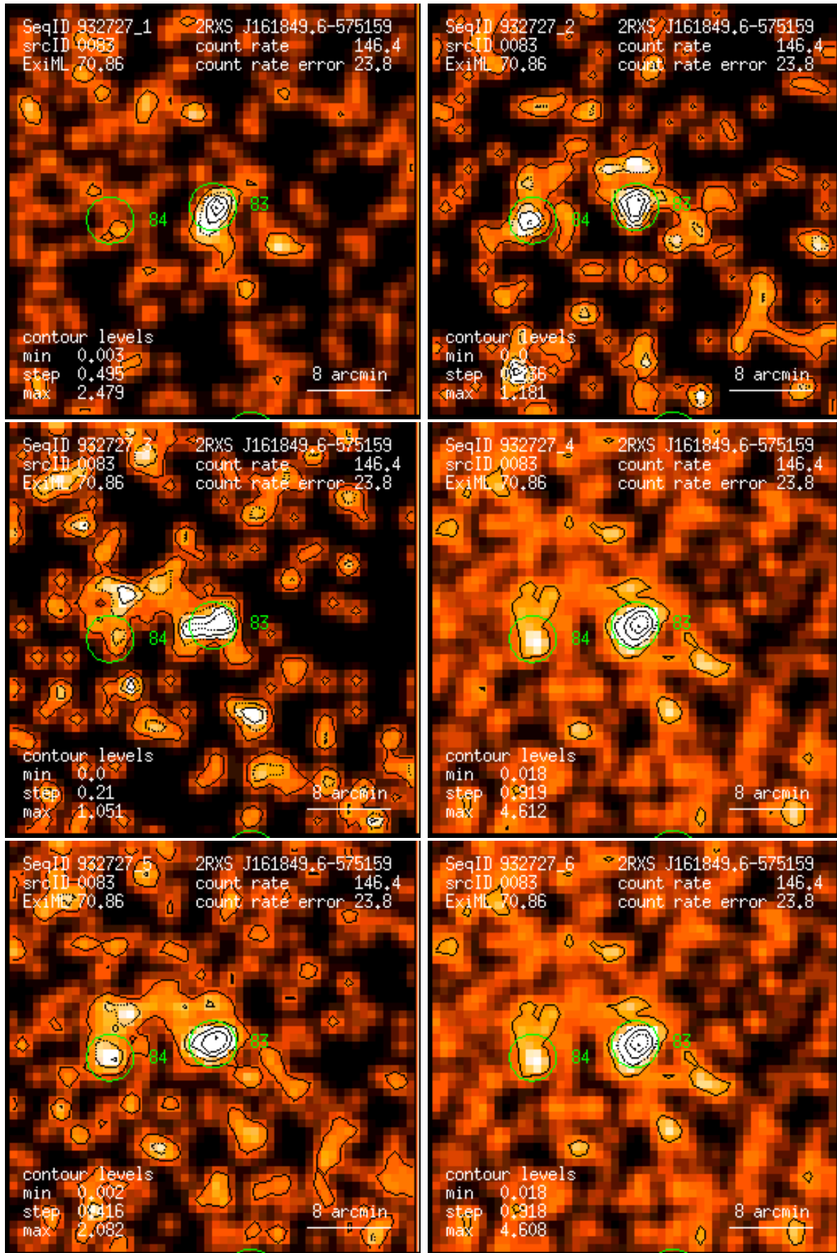
Figure 83: RASS 932727: detection 0083: band rate images, Gaussian filter: (1) PSPC channels 11 – 41, (2) 52 – 90, (3) 91 – 201, (4) 11 – 235, (5) 52 – 201, (6) 11 – 201. Broad band rates in counts/ks. Band rate contour levels in counts/ks/arcmin 2 .
