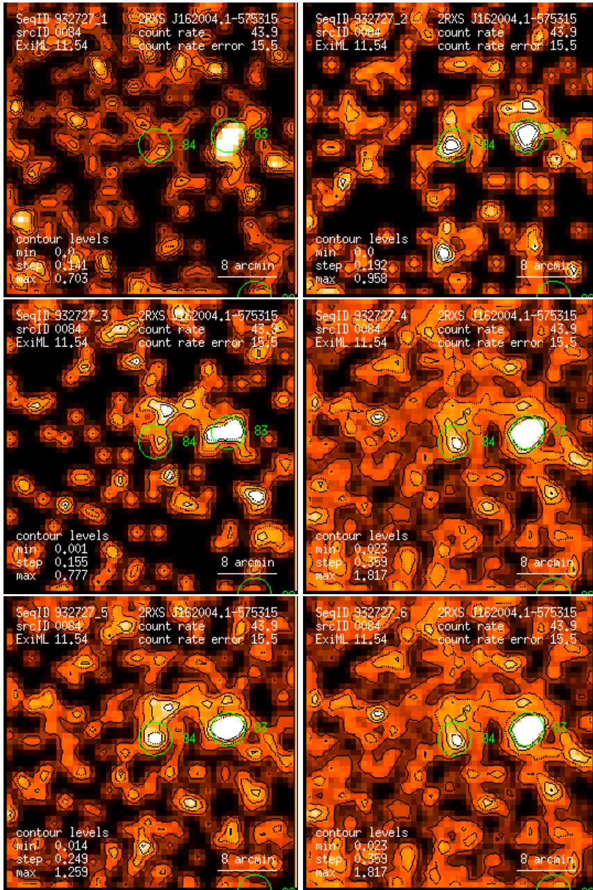
Figure 84: RASS 932727: detection 0084: band rate images, Gaussian filter: (1) PSPC channels 11 – 41, (2) 52 – 90, (3) 91 – 201, (4) 11 – 235, (5) 52 – 201, (6) 11 – 201. Broad band rates in counts/ks. Band rate contour levels in counts/ks/arcmin 2 .
