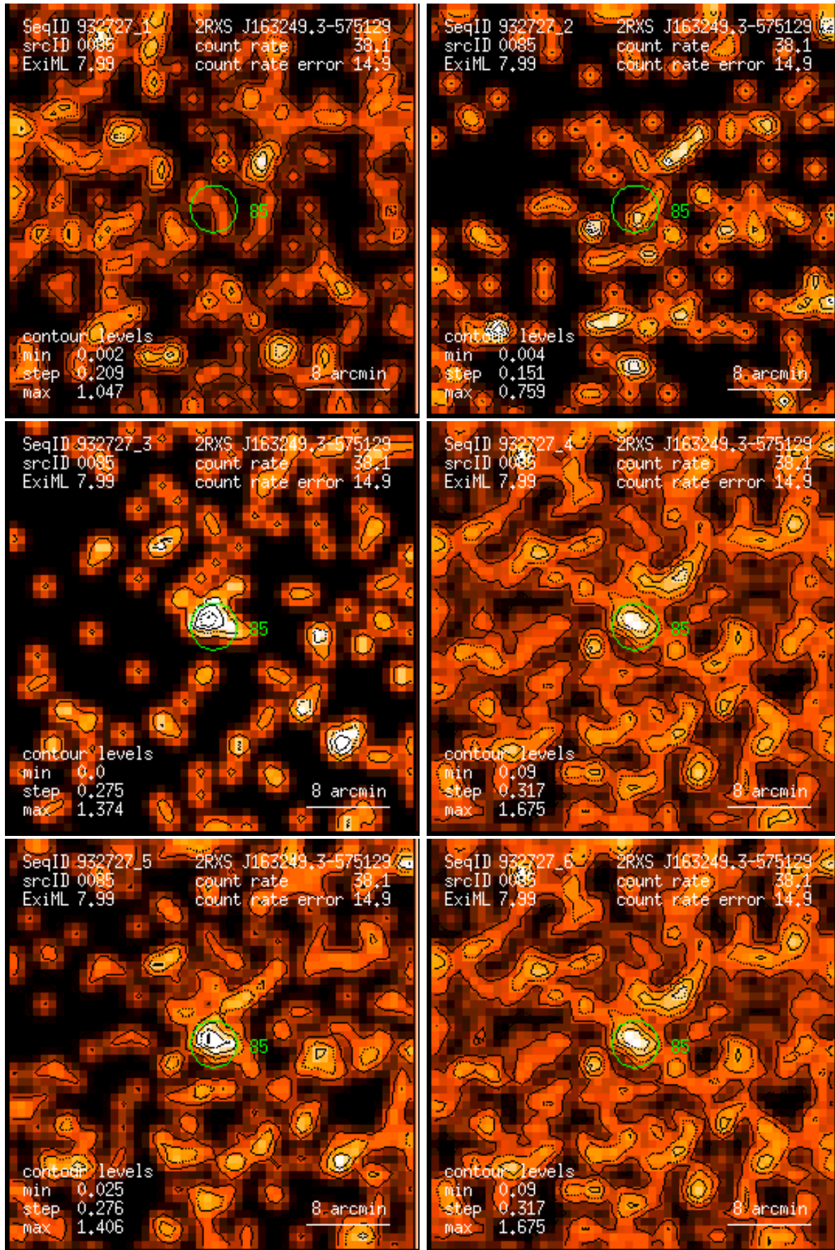
Figure 85: RASS 932727: detection 0085: band rate images, Gaussian filter: (1) PSPC channels 11 – 41, (2) 52 – 90, (3) 91 – 201, (4) 11 – 235, (5) 52 – 201, (6) 11 – 201. Broad band rates in counts/ks. Band rate contour levels in counts/ks/arcmin 2 .
