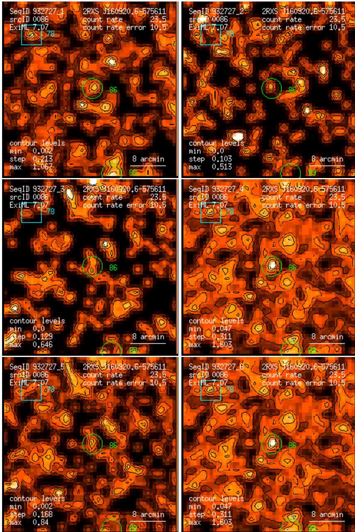
Figure 86: RASS 932727: detection 0086: band rate images, Gaussian filter: (1) PSPC channels 11 – 41, (2) 52 – 90, (3) 91 – 201, (4) 11 – 235, (5) 52 – 201, (6) 11 – 201. Broad band rates in counts/ks. Band rate contour levels in counts/ks/arcmin 2 .
