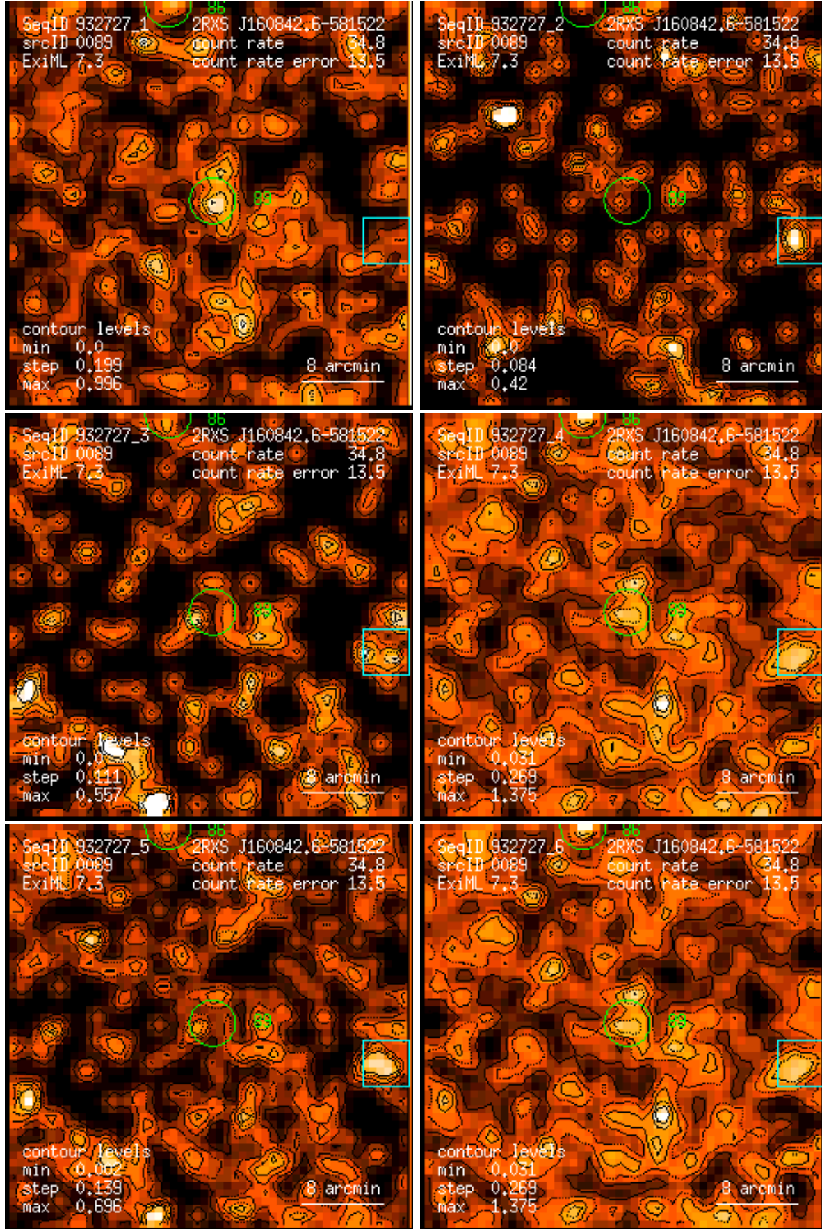
Figure 89: RASS 932727: detection 0089: band rate images, Gaussian filter: (1) PSPC channels 11 – 41, (2) 52 – 90, (3) 91 – 201, (4) 11 – 235, (5) 52 – 201, (6) 11 – 201. Broad band rates in counts/ks. Band rate contour levels in counts/ks/arcmin 2 .
