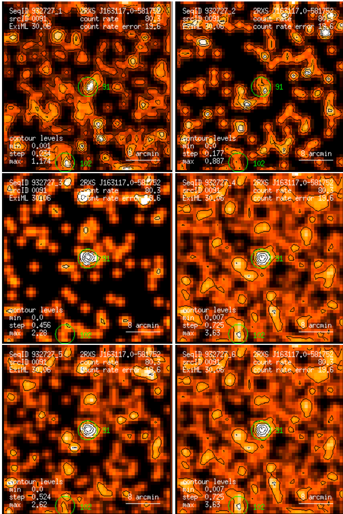
Figure 91: RASS 932727: detection 0091: band rate images, Gaussian filter: (1) PSPC channels 11 – 41, (2) 52 – 90, (3) 91 – 201, (4) 11 – 235, (5) 52 – 201, (6) 11 – 201. Broad band rates in counts/ks. Band rate contour levels in counts/ks/arcmin 2 .
