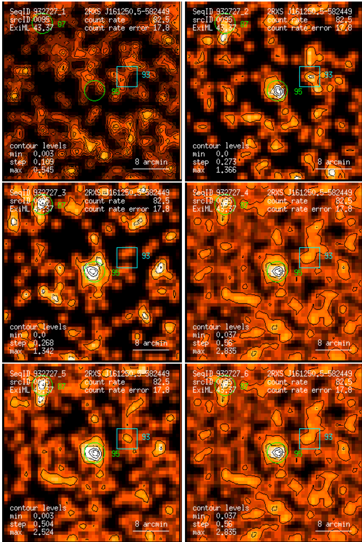
Figure 95: RASS 932727: detection 0095: band rate images, Gaussian filter: (1) PSPC channels 11 – 41, (2) 52 – 90, (3) 91 – 201, (4) 11 – 235, (5) 52 – 201, (6) 11 – 201. Broad band rates in counts/ks. Band rate contour levels in counts/ks/arcmin 2 .
