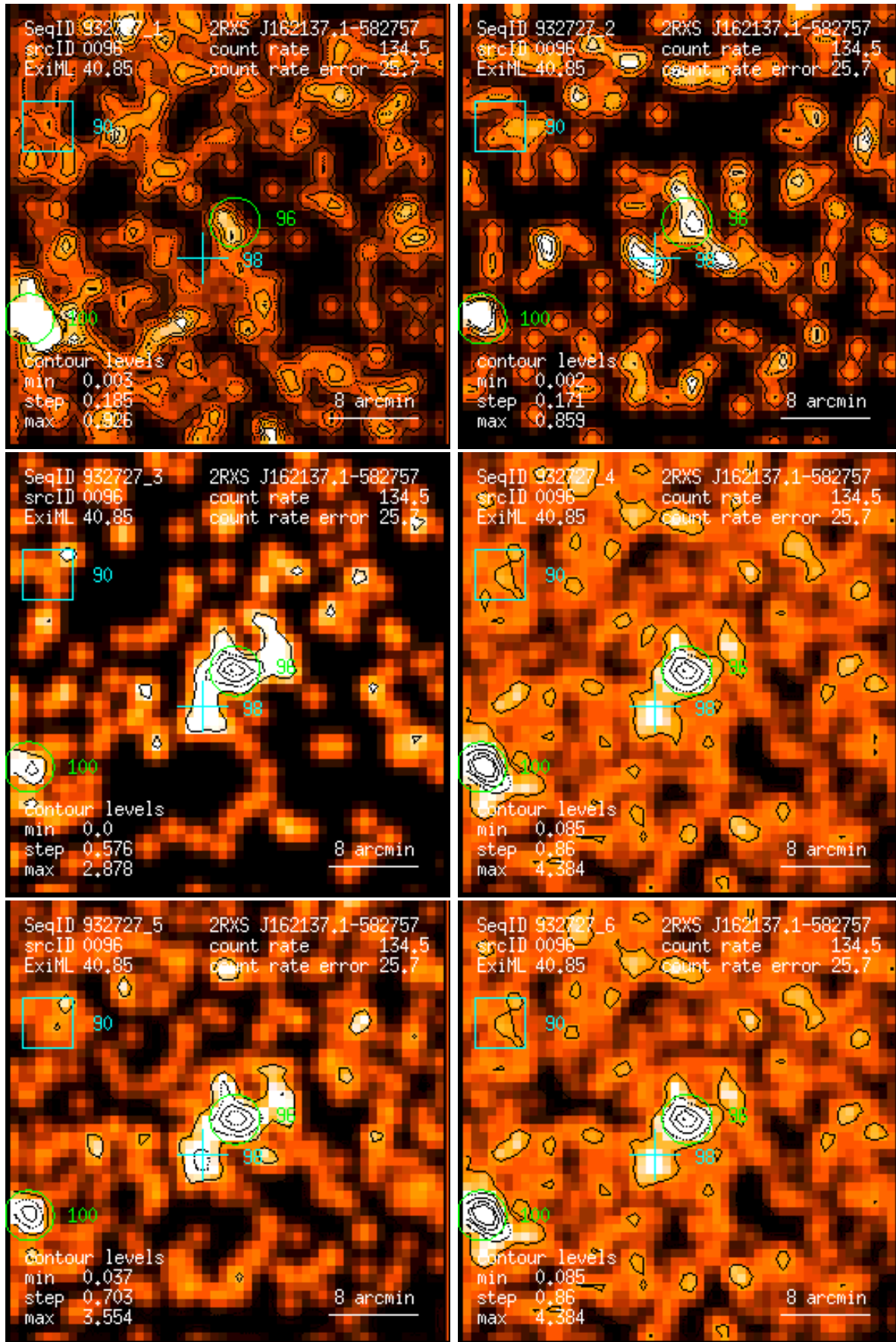
Figure 96: RASS 932727: detection 0096: band rate images, Gaussian filter: (1) PSPC channels 11 – 41, (2) 52 – 90, (3) 91 – 201, (4) 11 – 235, (5) 52 – 201, (6) 11 – 201. Broad band rates in counts/ks. Band rate contour levels in counts/ks/arcmin 2 .
