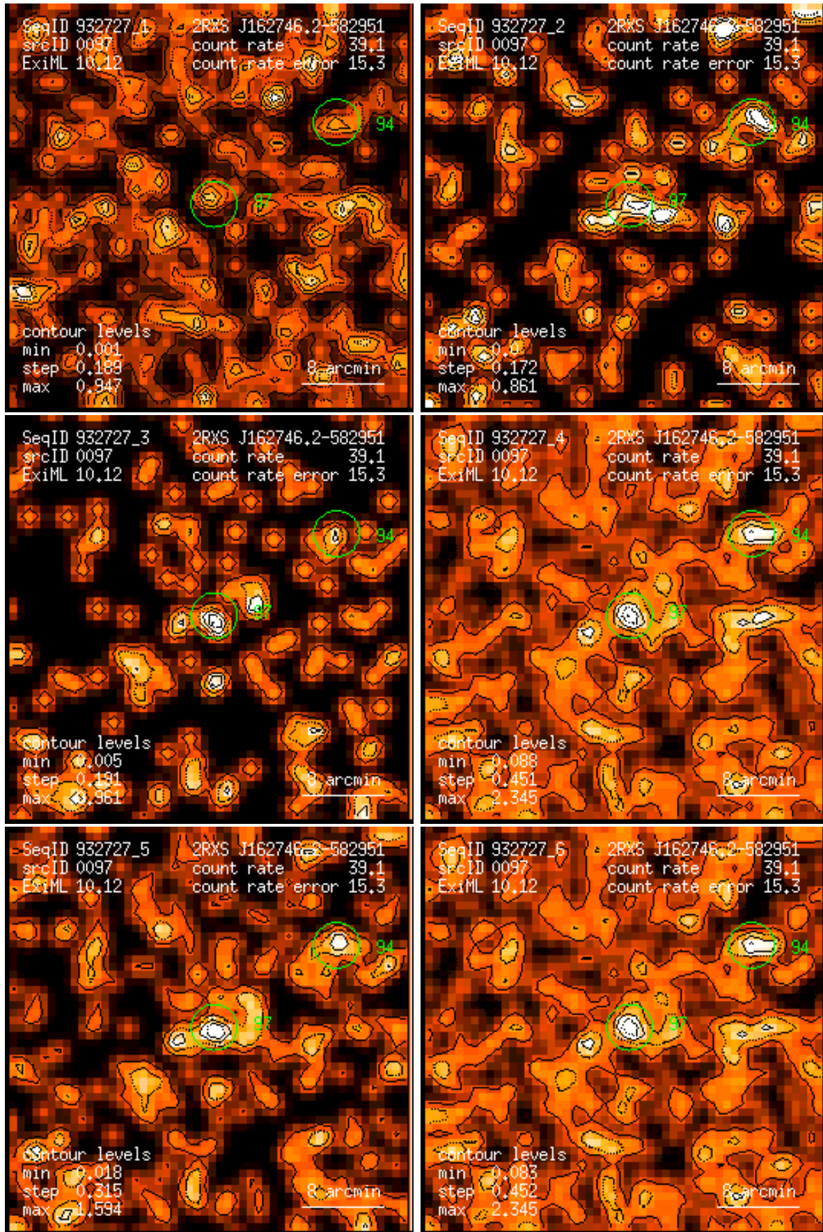
Figure 97: RASS 932727: detection 0097: band rate images, Gaussian filter: (1) PSPC channels 11 – 41, (2) 52 – 90, (3) 91 – 201, (4) 11 – 235, (5) 52 – 201, (6) 11 – 201. Broad band rates in counts/ks. Band rate contour levels in counts/ks/arcmin 2 .
