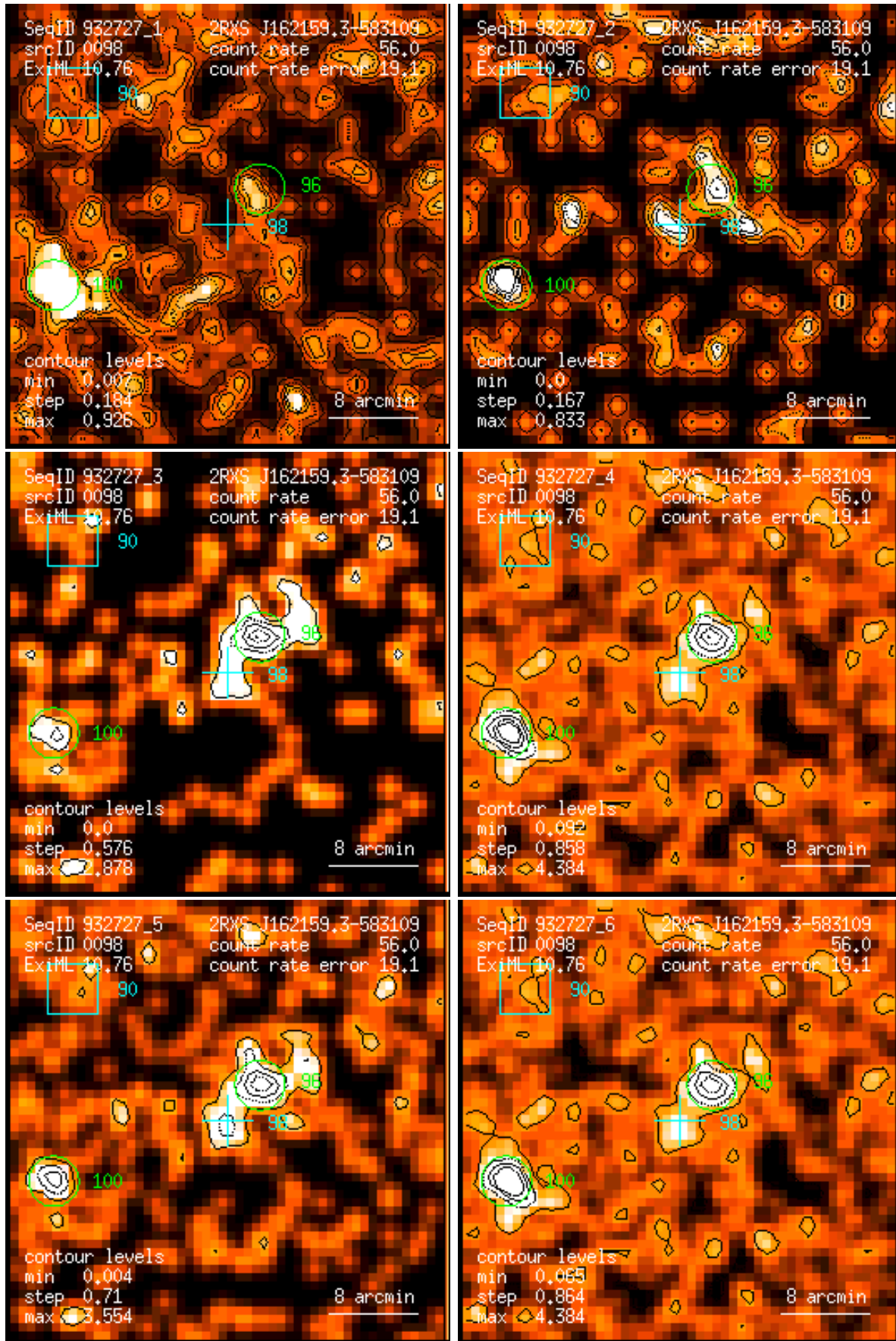
Figure 98: RASS 932727: detection 0098: band rate images, Gaussian filter: (1) PSPC channels 11 – 41, (2) 52 – 90, (3) 91 – 201, (4) 11 – 235, (5) 52 – 201, (6) 11 – 201. Broad band rates in counts/ks. Band rate contour levels in counts/ks/arcmin 2 .
