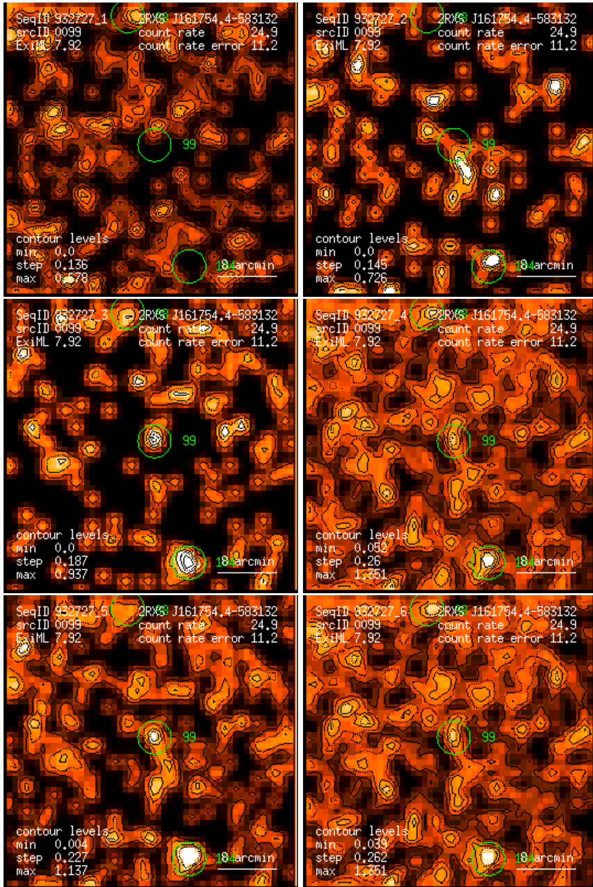
Figure 99: RASS 932727: detection 0099: band rate images, Gaussian filter: (1) PSPC channels 11 – 41, (2) 52 – 90, (3) 91 – 201, (4) 11 – 235, (5) 52 – 201, (6) 11 – 201. Broad band rates in counts/ks. Band rate contour levels in counts/ks/arcmin 2 .
