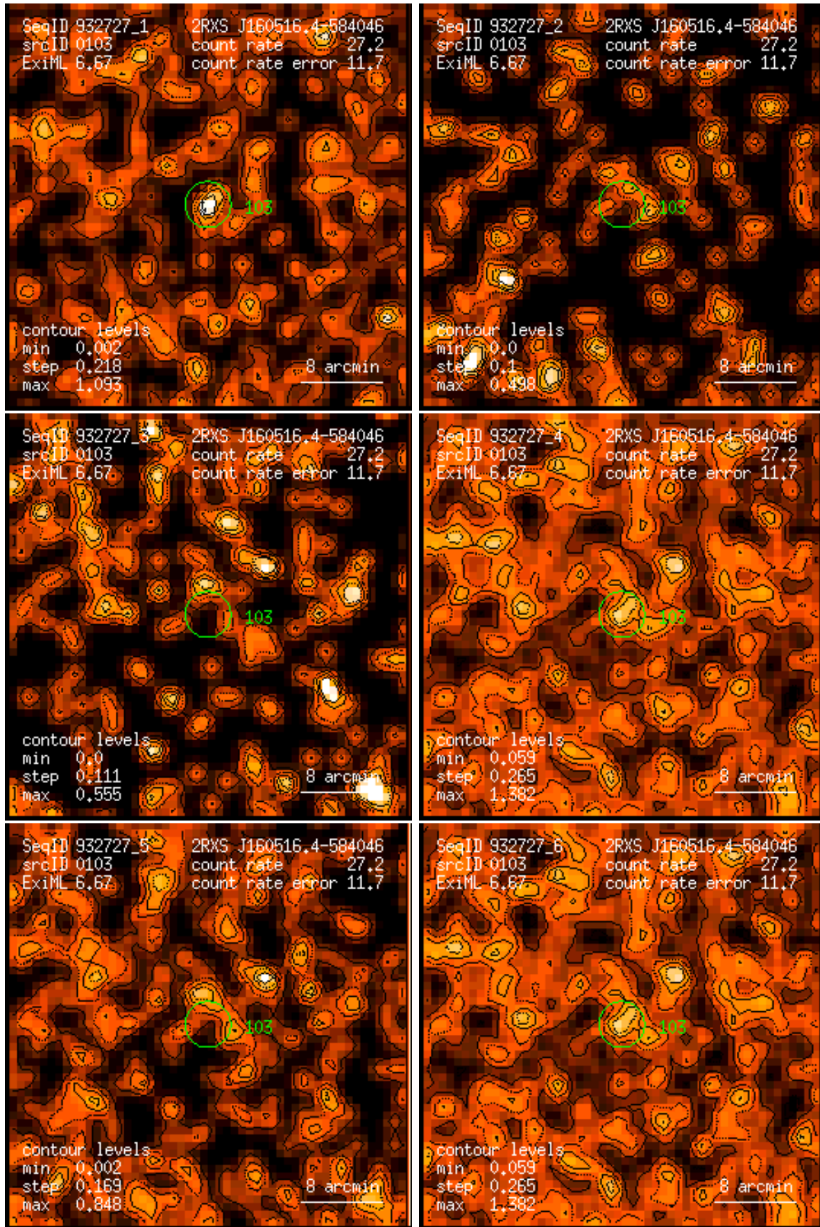
Figure 103: RASS 932727: detection 0103: band rate images, Gaussian filter: (1) PSPC channels 11 – 41, (2) 52 – 90, (3) 91 – 201, (4) 11 – 235, (5) 52 – 201, (6) 11 – 201. Broad band rates in counts/ks. Band rate contour levels in counts/ks/arcmin 2 .
