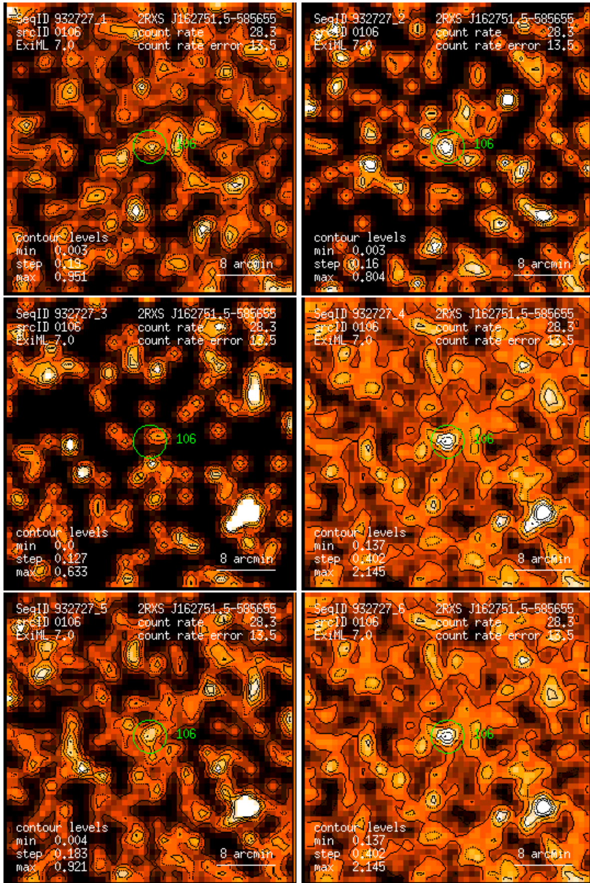
Figure 106: RASS 932727: detection 0106: band rate images, Gaussian filter: (1) PSPC channels 11 – 41, (2) 52 – 90, (3) 91 – 201, (4) 11 – 235, (5) 52 – 201, (6) 11 – 201. Broad band rates in counts/ks. Band rate contour levels in counts/ks/arcmin 2 .
