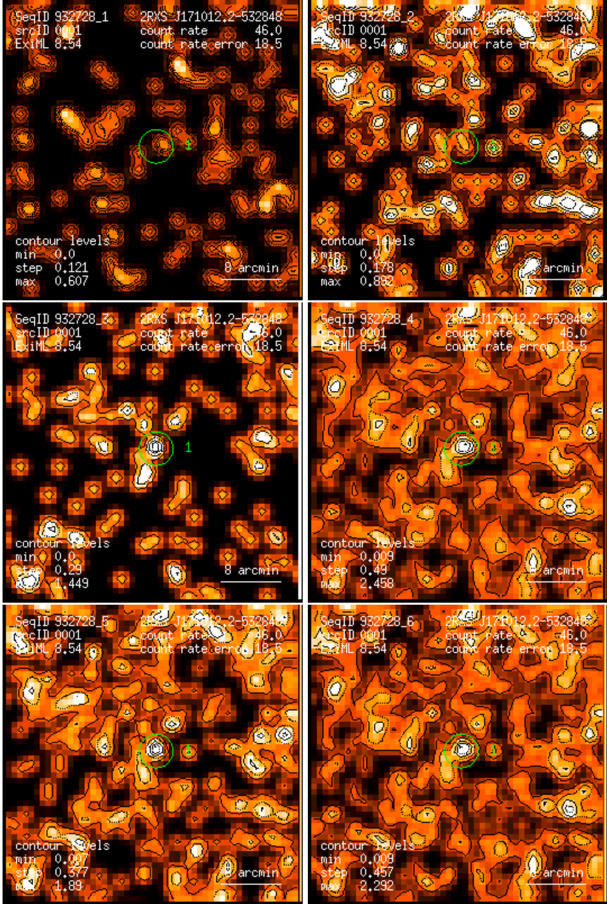
Figure 1: RASS 932728: detection 0001: band rate images, Gaussian filter: (1) PSPC channels 11 – 41, (2) 52 – 90, (3) 91 – 201, (4) 11 – 235, (5) 52 – 201, (6) 11 – 201. Broad band rates in counts/ks. Band rate contour levels in counts/ks/arcmin 2 .
