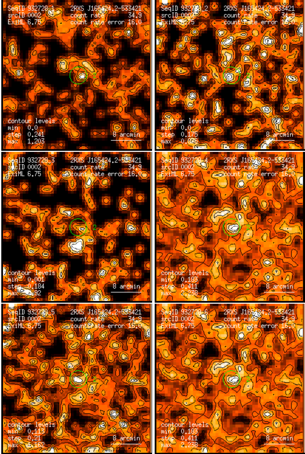
Figure 2: RASS 932728: detection 0002: band rate images, Gaussian filter: (1) PSPC channels 11 – 41, (2) 52 – 90, (3) 91 – 201, (4) 11 – 235, (5) 52 – 201, (6) 11 – 201. Broad band rates in counts/ks. Band rate contour levels in counts/ks/arcmin 2 .
