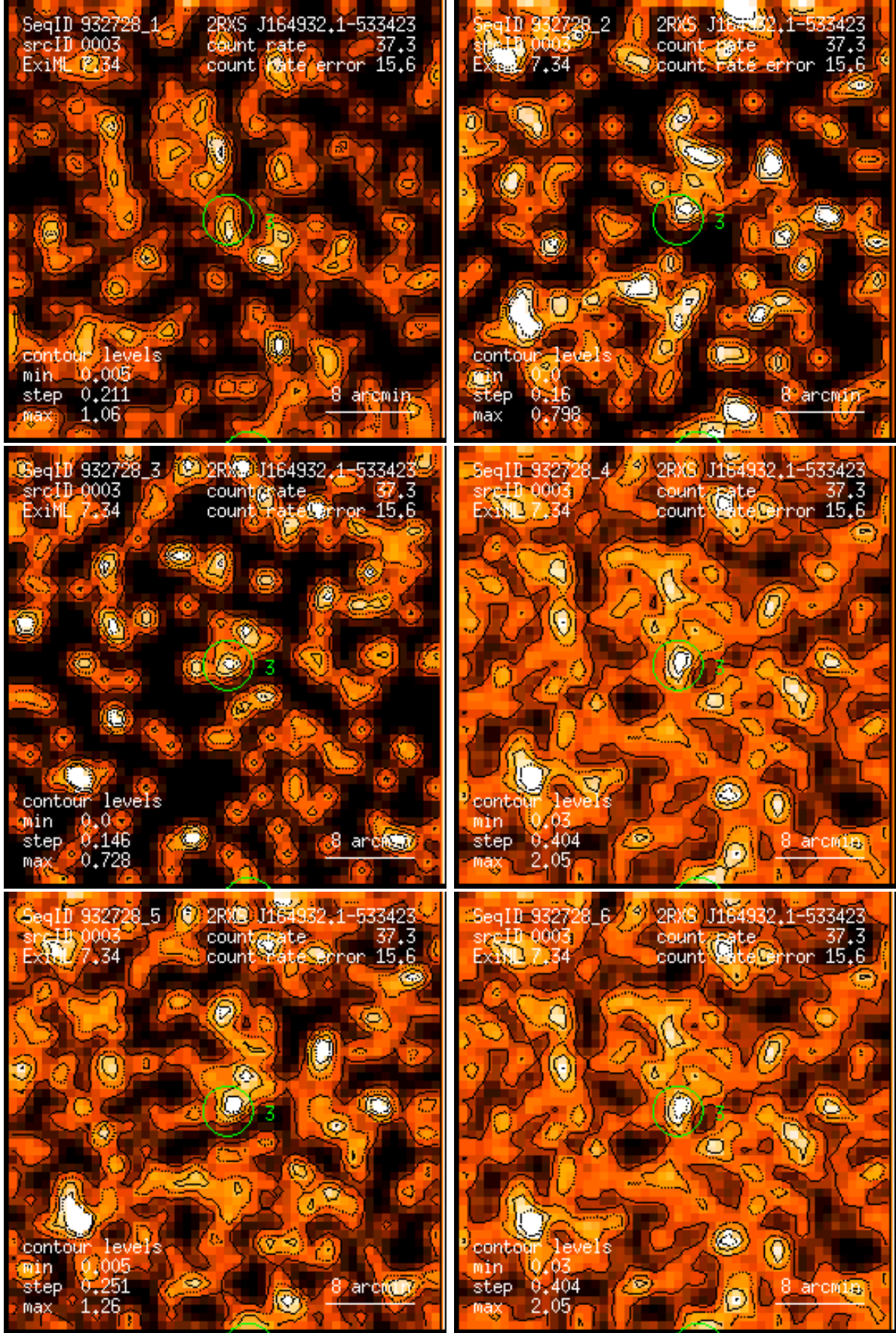
Figure 3: RASS 932728: detection 0003: band rate images, Gaussian filter: (1) PSPC channels 11 – 41, (2) 52 – 90, (3) 91 – 201, (4) 11 – 235, (5) 52 – 201, (6) 11 – 201. Broad band rates in counts/ks. Band rate contour levels in counts/ks/arcmin 2 .
