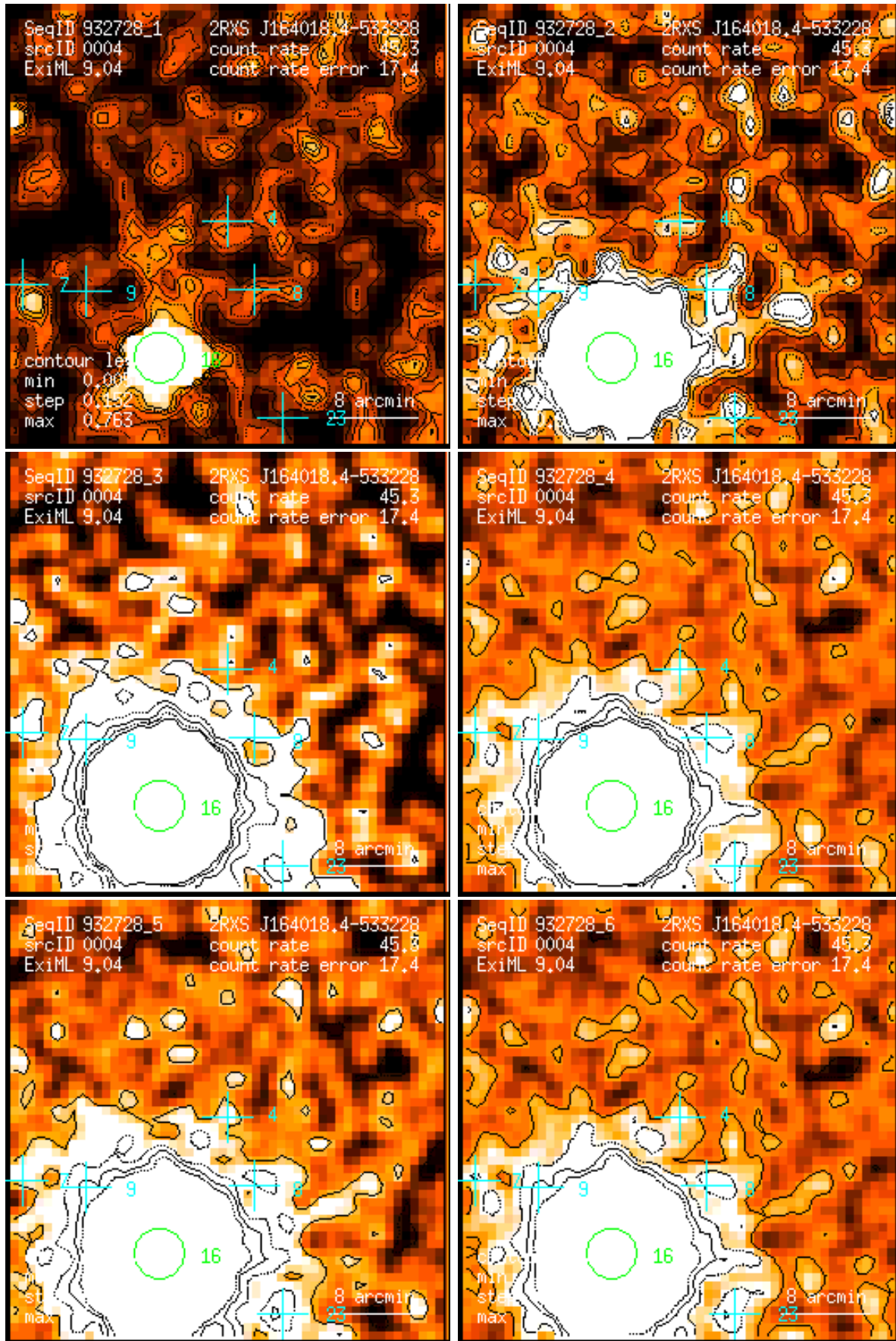
Figure 4: RASS 932728: detection 0004: band rate images, Gaussian filter: (1) PSPC channels 11 – 41, (2) 52 – 90, (3) 91 – 201, (4) 11 – 235, (5) 52 – 201, (6) 11 – 201. Broad band rates in counts/ks. Band rate contour levels in counts/ks/arcmin 2 .
