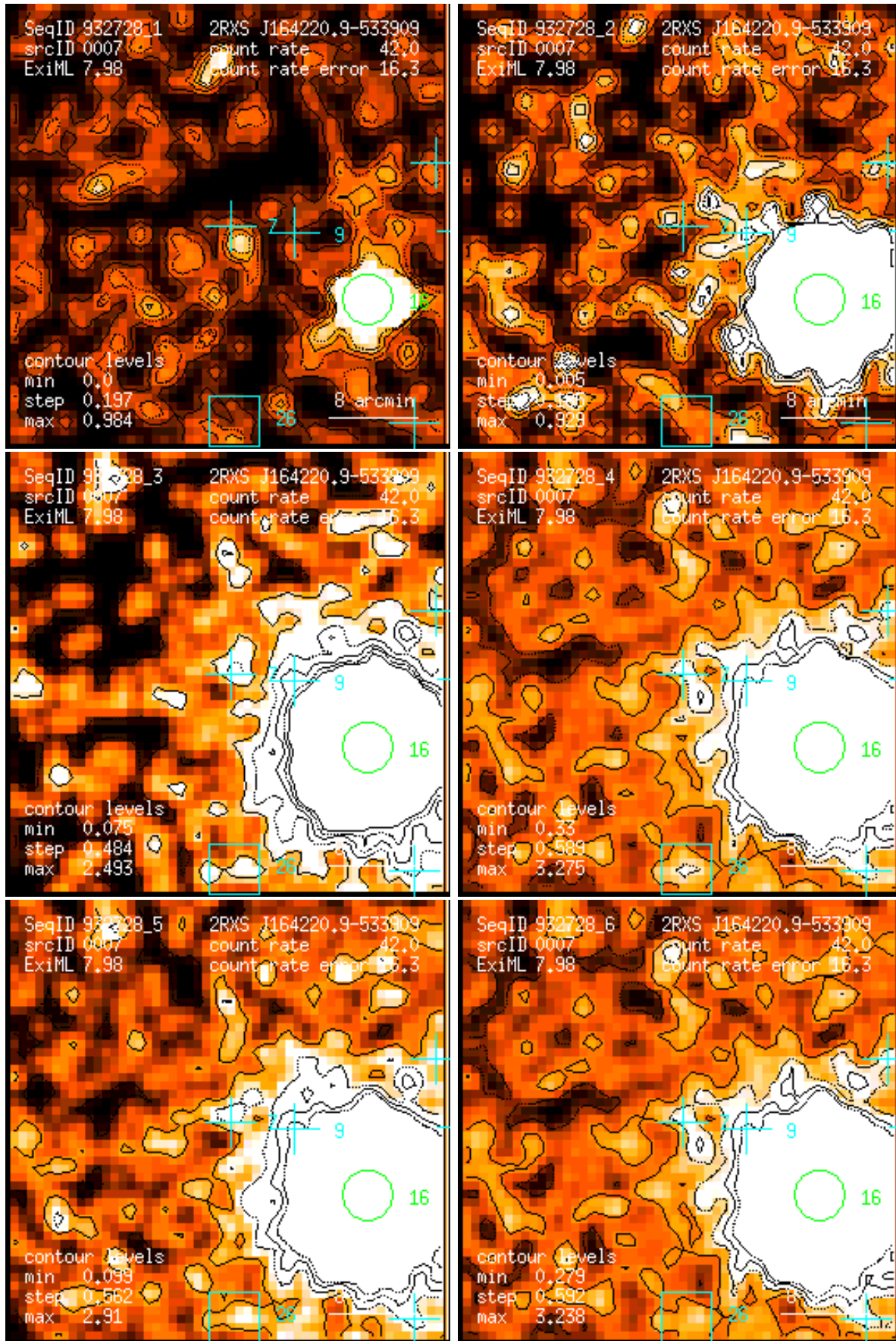
Figure 7: RASS 932728: detection 0007: band rate images, Gaussian filter: (1) PSPC channels 11 – 41, (2) 52 – 90, (3) 91 – 201, (4) 11 – 235, (5) 52 – 201, (6) 11 – 201. Broad band rates in counts/ks. Band rate contour levels in counts/ks/arcmin 2 .
