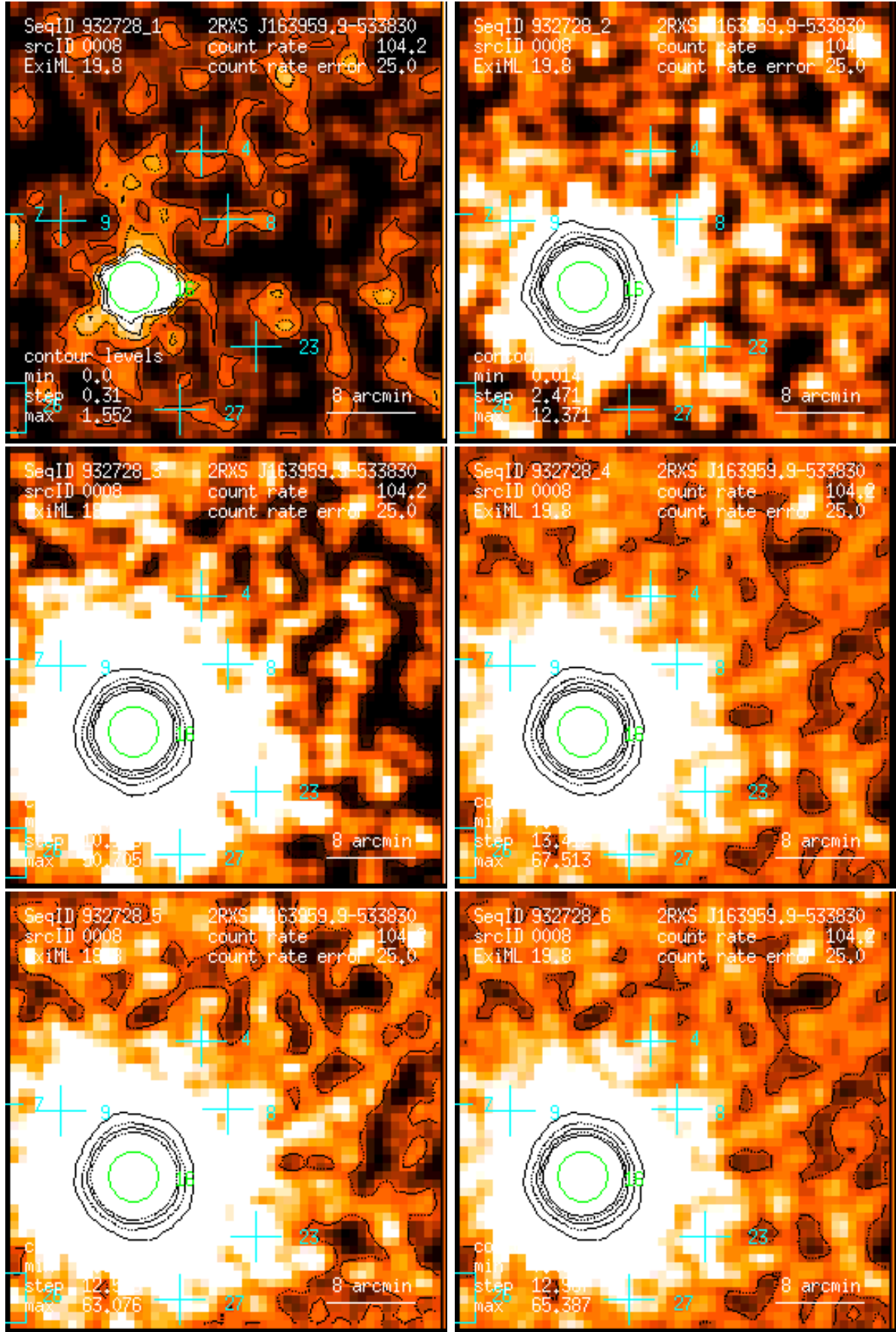
Figure 8: RASS 932728: detection 0008: band rate images, Gaussian filter: (1) PSPC channels 11 – 41, (2) 52 – 90, (3) 91 – 201, (4) 11 – 235, (5) 52 – 201, (6) 11 – 201. Broad band rates in counts/ks. Band rate contour levels in counts/ks/arcmin 2 .
