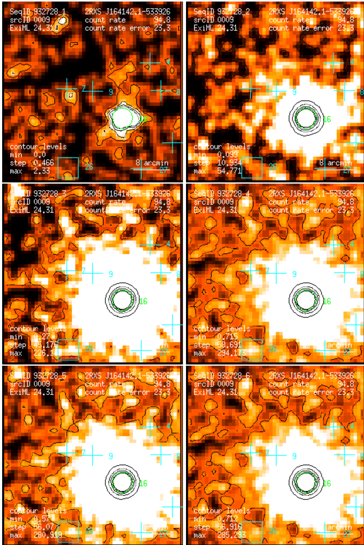
Figure 9: RASS 932728: detection 0009: band rate images, Gaussian filter: (1) PSPC channels 11 – 41, (2) 52 – 90, (3) 91 – 201, (4) 11 – 235, (5) 52 – 201, (6) 11 – 201. Broad band rates in counts/ks. Band rate contour levels in counts/ks/arcmin 2 .
