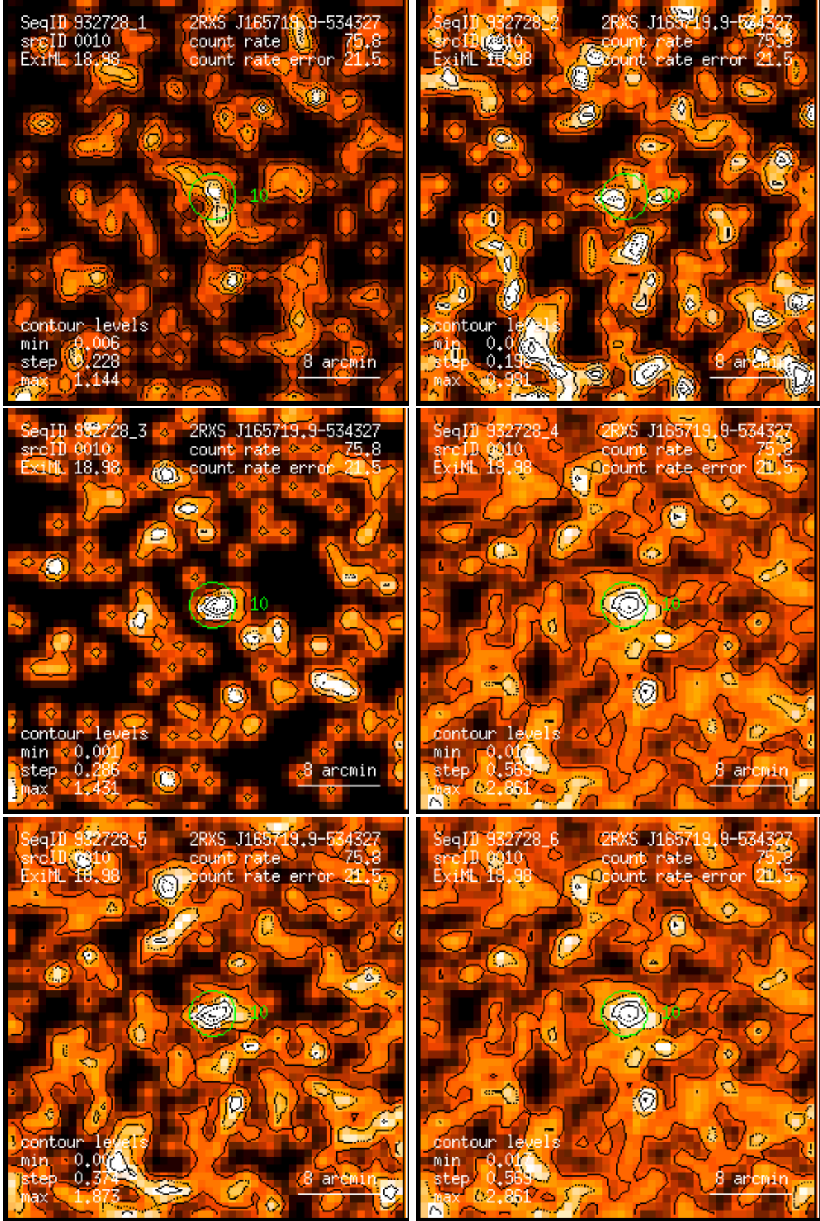
Figure 10: RASS 932728: detection 0010: band rate images, Gaussian filter: (1) PSPC channels 11 – 41, (2) 52 – 90, (3) 91 – 201, (4) 11 – 235, (5) 52 – 201, (6) 11 – 201. Broad band rates in counts/ks. Band rate contour levels in counts/ks/arcmin 2 .
