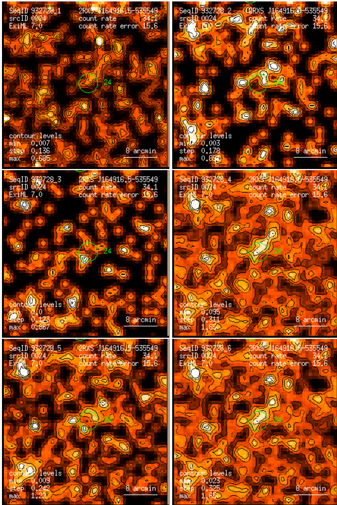
Figure 24: RASS 932728: detection 0024: band rate images, Gaussian filter: (1) PSPC channels 11 – 41, (2) 52 – 90, (3) 91 – 201, (4) 11 – 235, (5) 52 – 201, (6) 11 – 201. Broad band rates in counts/ks. Band rate contour levels in counts/ks/arcmin 2 .
