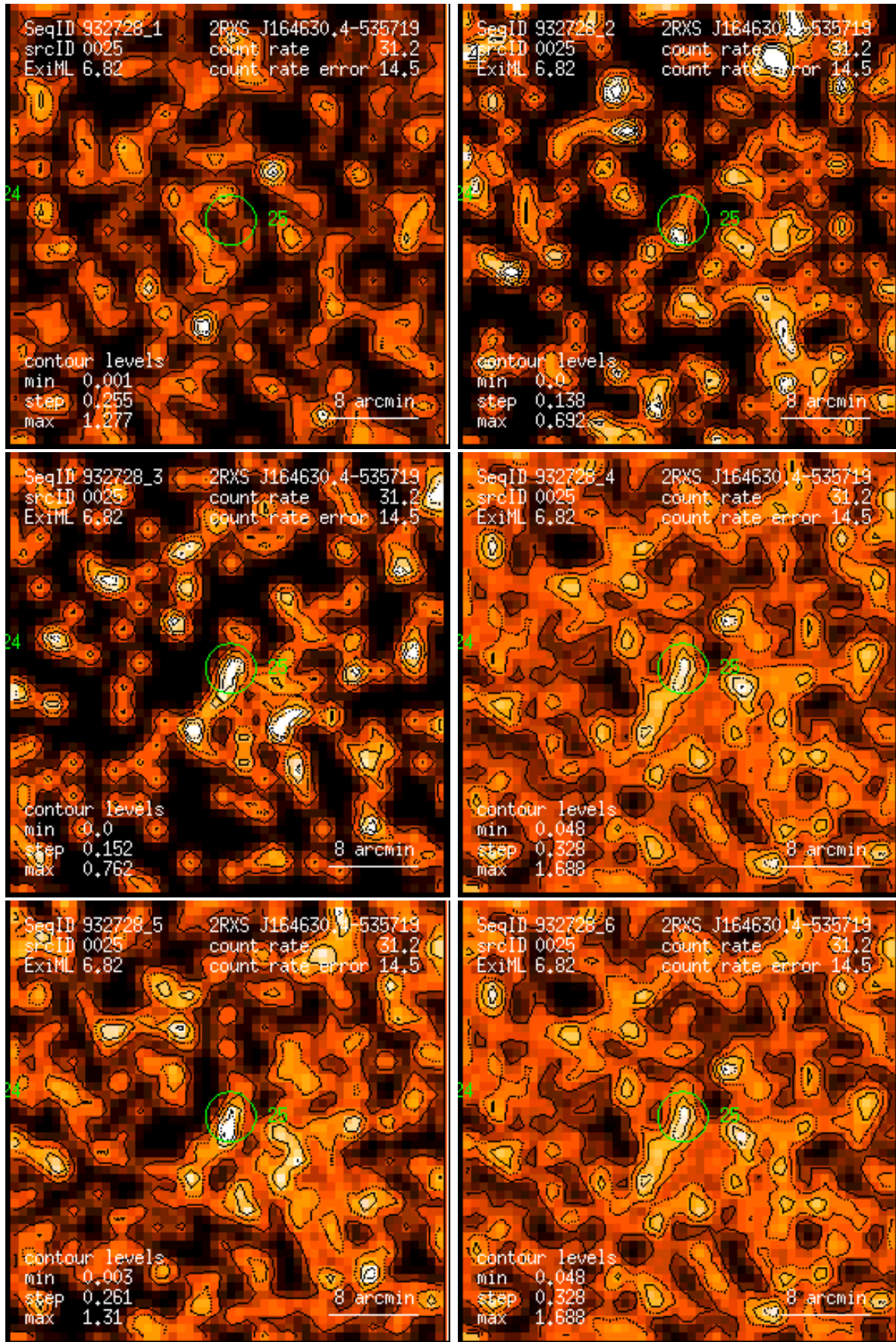
Figure 25: RASS 932728: detection 0025: band rate images, Gaussian filter: (1) PSPC channels 11 – 41, (2) 52 – 90, (3) 91 – 201, (4) 11 – 235, (5) 52 – 201, (6) 11 – 201. Broad band rates in counts/ks. Band rate contour levels in counts/ks/arcmin 2 .
