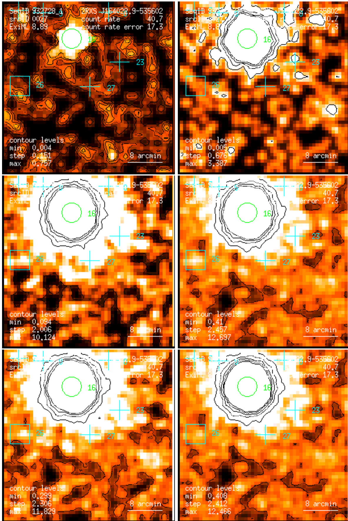
Figure 27: RASS 932728: detection 0027: band rate images, Gaussian filter: (1) PSPC channels 11 – 41, (2) 52 – 90, (3) 91 – 201, (4) 11 – 235, (5) 52 – 201, (6) 11 – 201. Broad band rates in counts/ks. Band rate contour levels in counts/ks/arcmin 2 .
