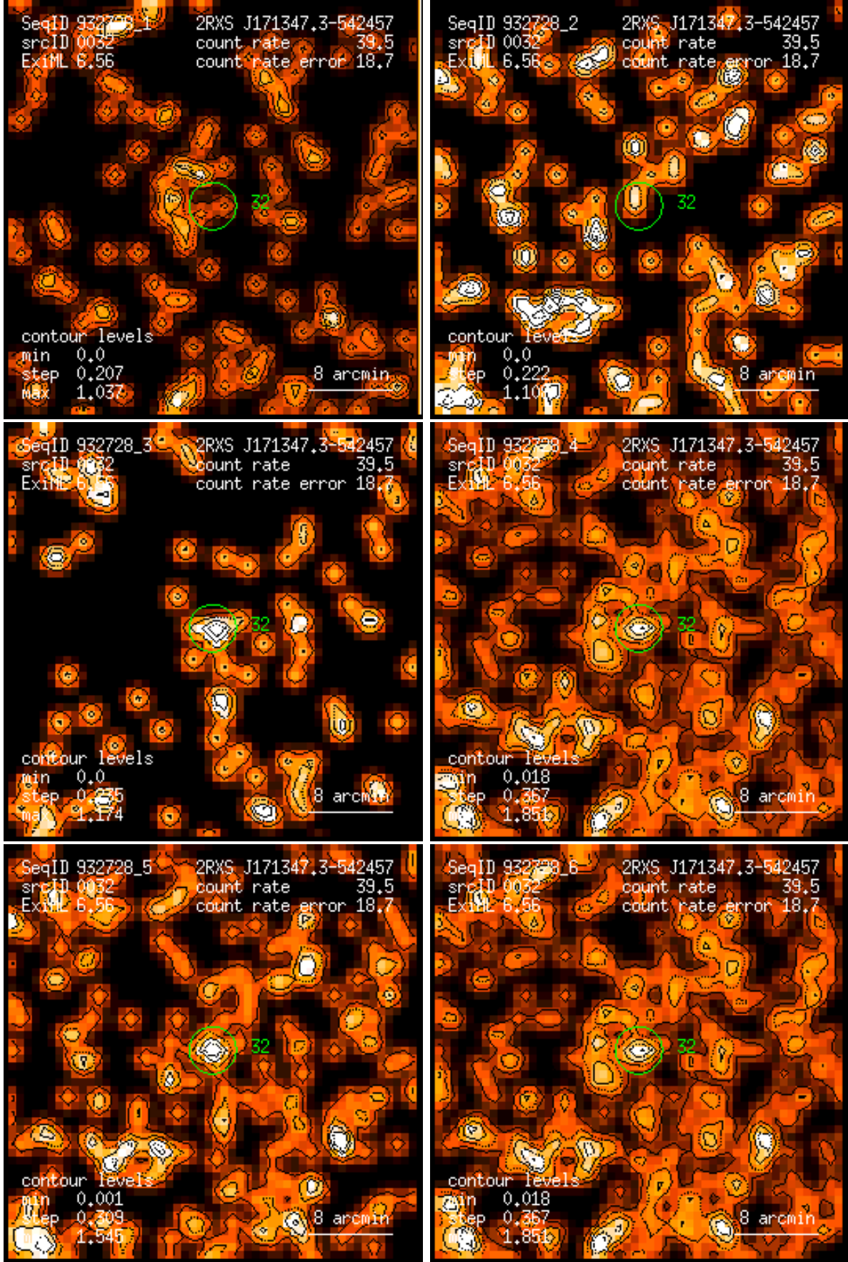
Figure 32: RASS 932728: detection 0032: band rate images, Gaussian filter: (1) PSPC channels 11 – 41, (2) 52 – 90, (3) 91 – 201, (4) 11 – 235, (5) 52 – 201, (6) 11 – 201. Broad band rates in counts/ks. Band rate contour levels in counts/ks/arcmin 2 .
