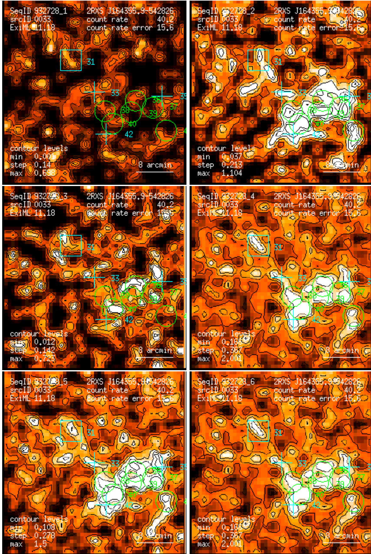
Figure 33: RASS 932728: detection 0033: band rate images, Gaussian filter: (1) PSPC channels 11 – 41, (2) 52 – 90, (3) 91 – 201, (4) 11 – 235, (5) 52 – 201, (6) 11 – 201. Broad band rates in counts/ks. Band rate contour levels in counts/ks/arcmin 2 .
