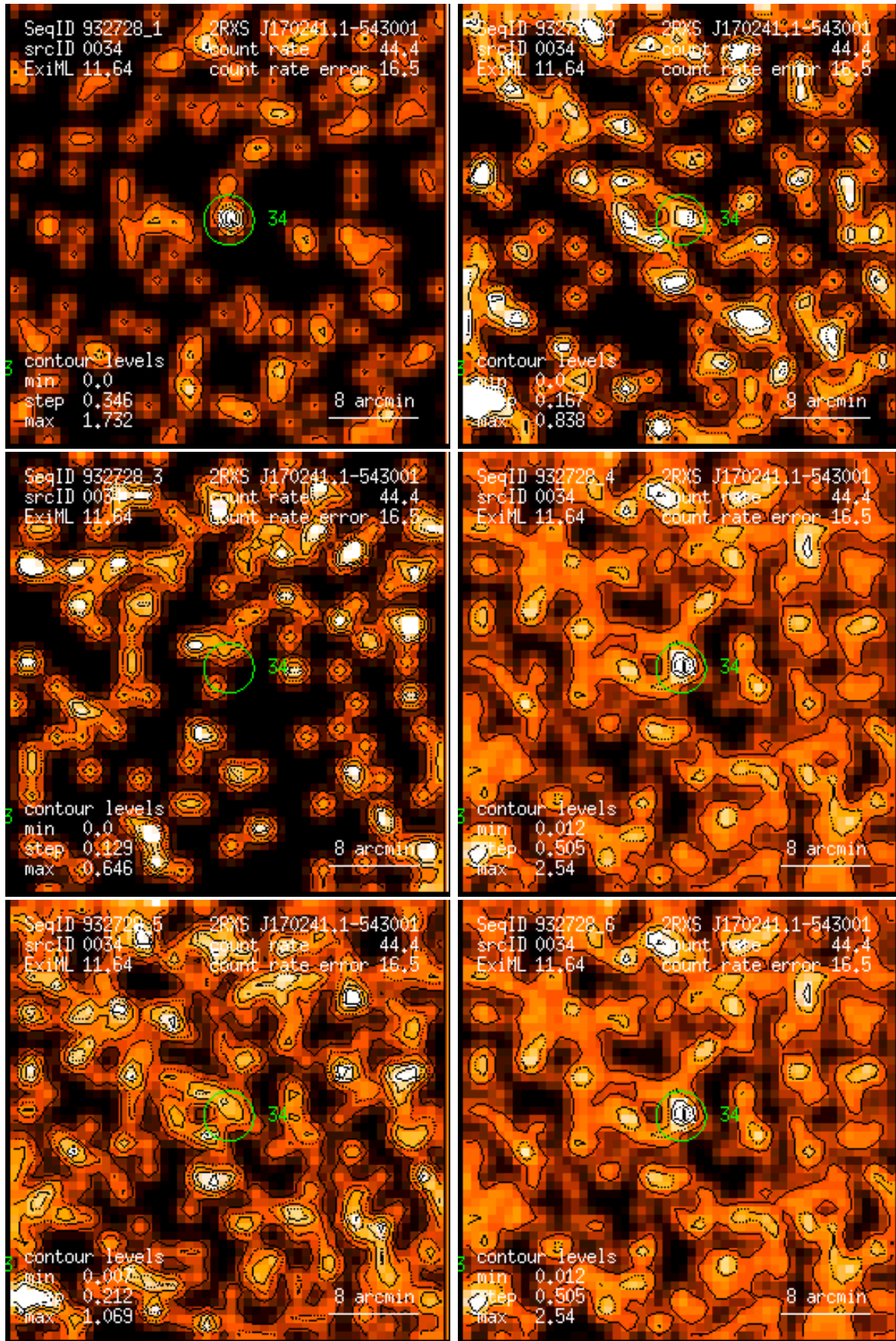
Figure 34: RASS 932728: detection 0034: band rate images, Gaussian filter: (1) PSPC channels 11 – 41, (2) 52 – 90, (3) 91 – 201, (4) 11 – 235, (5) 52 – 201, (6) 11 – 201. Broad band rates in counts/ks. Band rate contour levels in counts/ks/arcmin 2 .
