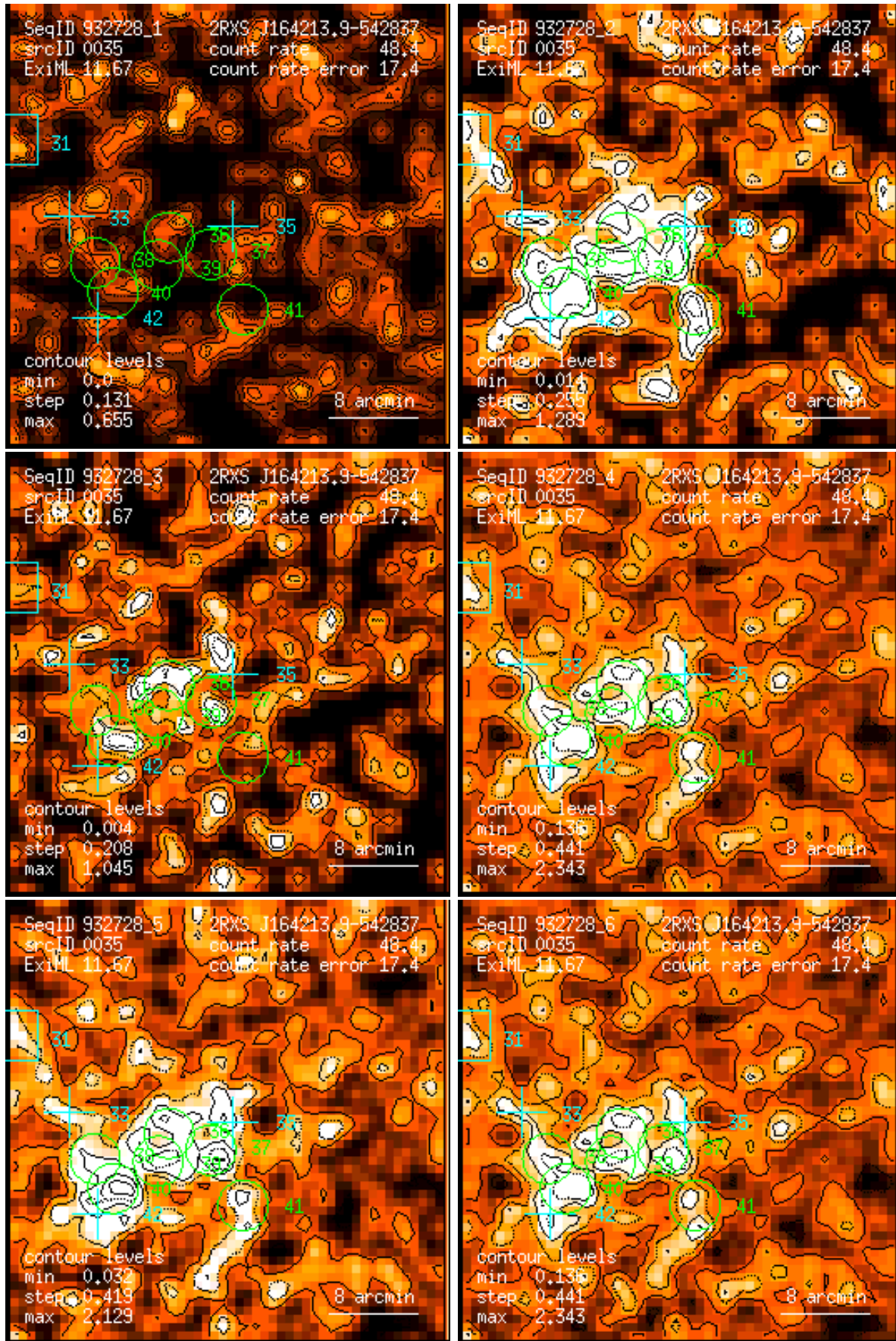
Figure 35: RASS 932728: detection 0035: band rate images, Gaussian filter: (1) PSPC channels 11 – 41, (2) 52 – 90, (3) 91 – 201, (4) 11 – 235, (5) 52 – 201, (6) 11 – 201. Broad band rates in counts/ks. Band rate contour levels in counts/ks/arcmin 2 .
