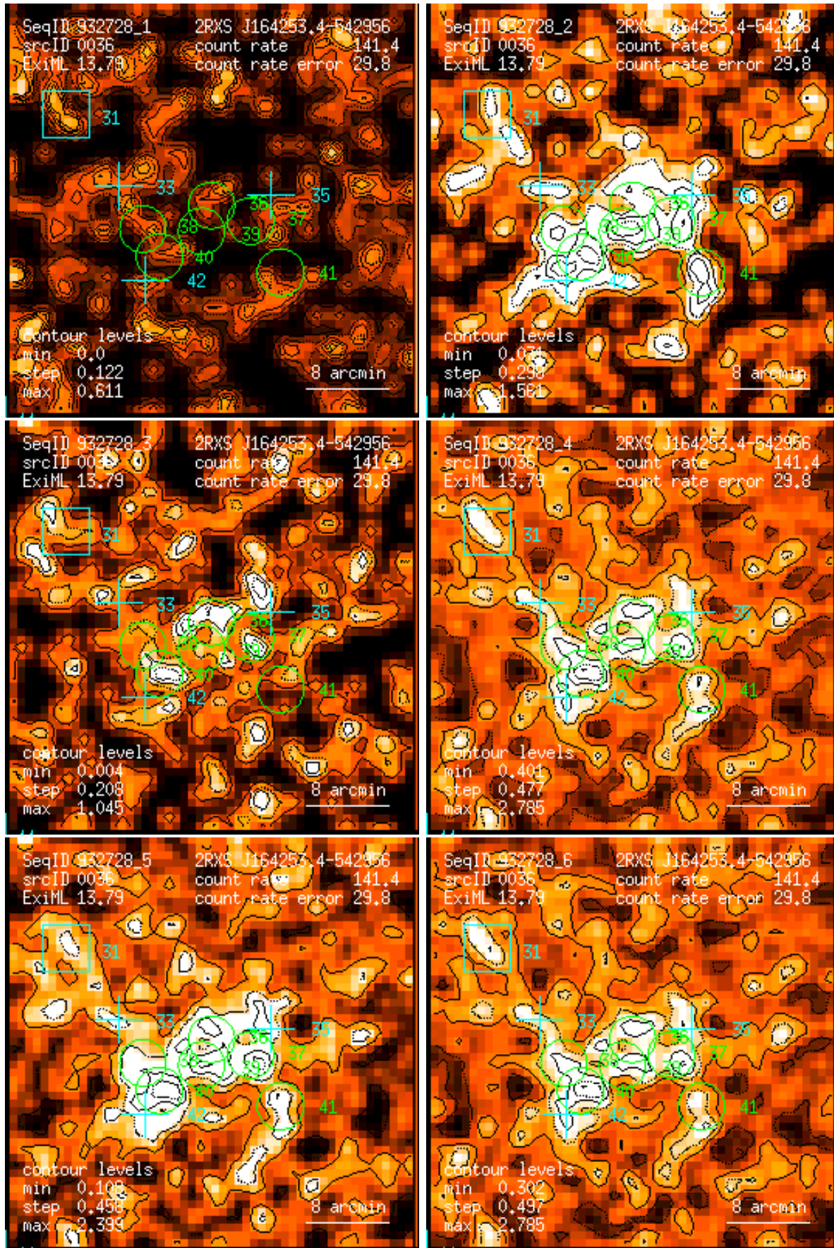
Figure 36: RASS 932728: detection 0036: band rate images, Gaussian filter: (1) PSPC channels 11 – 41, (2) 52 – 90, (3) 91 – 201, (4) 11 – 235, (5) 52 – 201, (6) 11 – 201. Broad band rates in counts/ks. Band rate contour levels in counts/ks/arcmin 2 .
