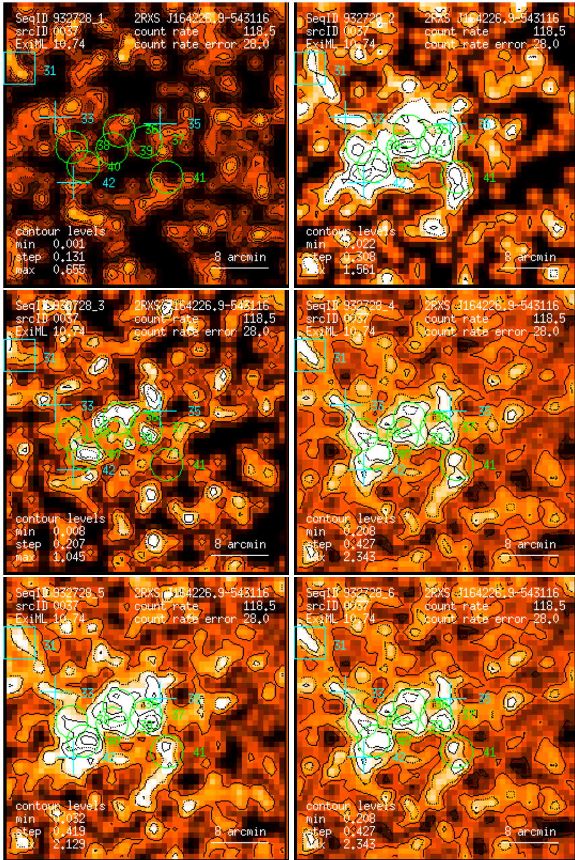
Figure 37: RASS 932728: detection 0037: band rate images, Gaussian filter: (1) PSPC channels 11 – 41, (2) 52 – 90, (3) 91 – 201, (4) 11 – 235, (5) 52 – 201, (6) 11 – 201. Broad band rates in counts/ks. Band rate contour levels in counts/ks/arcmin 2 .
