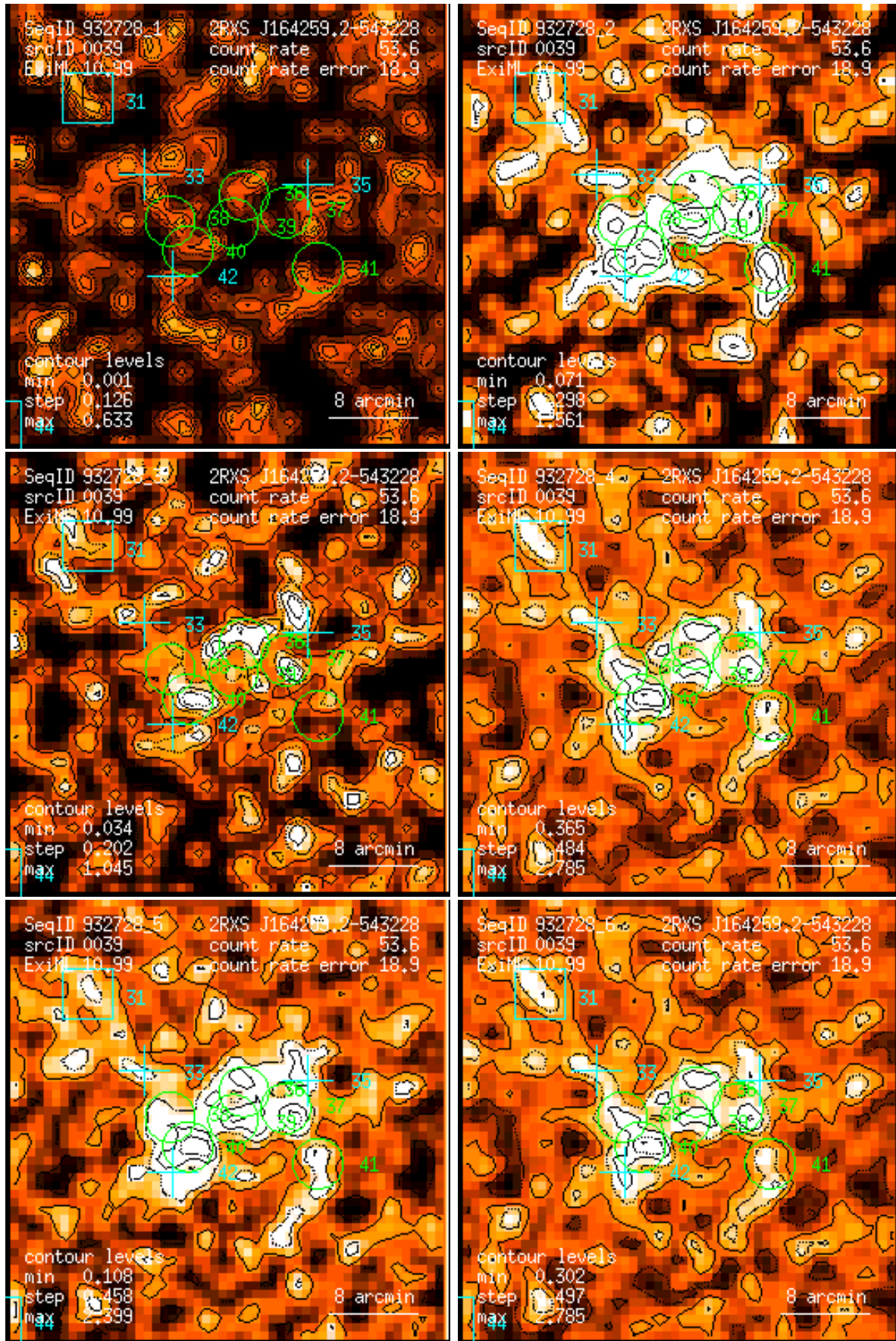
Figure 39: RASS 932728: detection 0039: band rate images, Gaussian filter: (1) PSPC channels 11 – 41, (2) 52 – 90, (3) 91 – 201, (4) 11 – 235, (5) 52 – 201, (6) 11 – 201. Broad band rates in counts/ks. Band rate contour levels in counts/ks/arcmin 2 .
