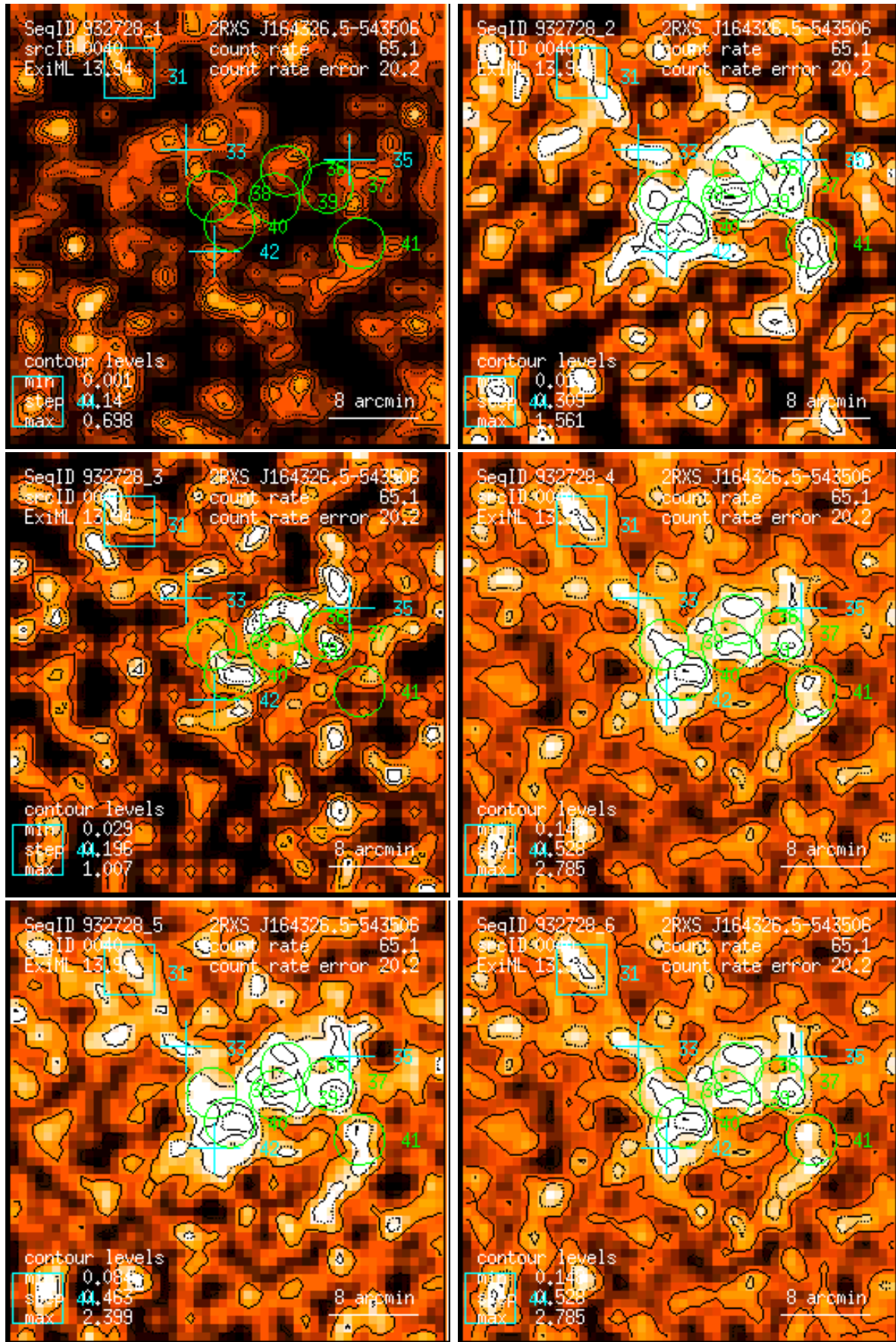
Figure 40: RASS 932728: detection 0040: band rate images, Gaussian filter: (1) PSPC channels 11 – 41, (2) 52 – 90, (3) 91 – 201, (4) 11 – 235, (5) 52 – 201, (6) 11 – 201. Broad band rates in counts/ks. Band rate contour levels in counts/ks/arcmin 2 .
