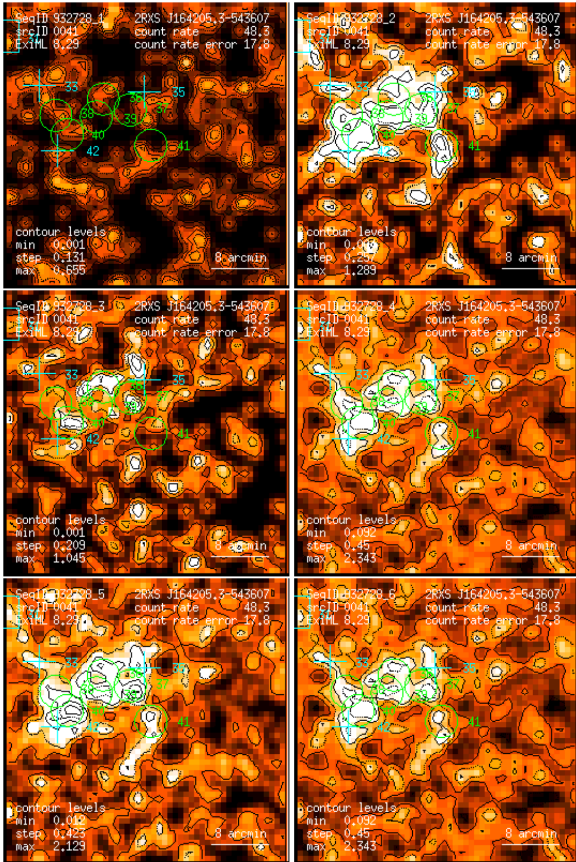
Figure 41: RASS 932728: detection 0041: band rate images, Gaussian filter: (1) PSPC channels 11 – 41, (2) 52 – 90, (3) 91 – 201, (4) 11 – 235, (5) 52 – 201, (6) 11 – 201. Broad band rates in counts/ks. Band rate contour levels in counts/ks/arcmin 2 .
