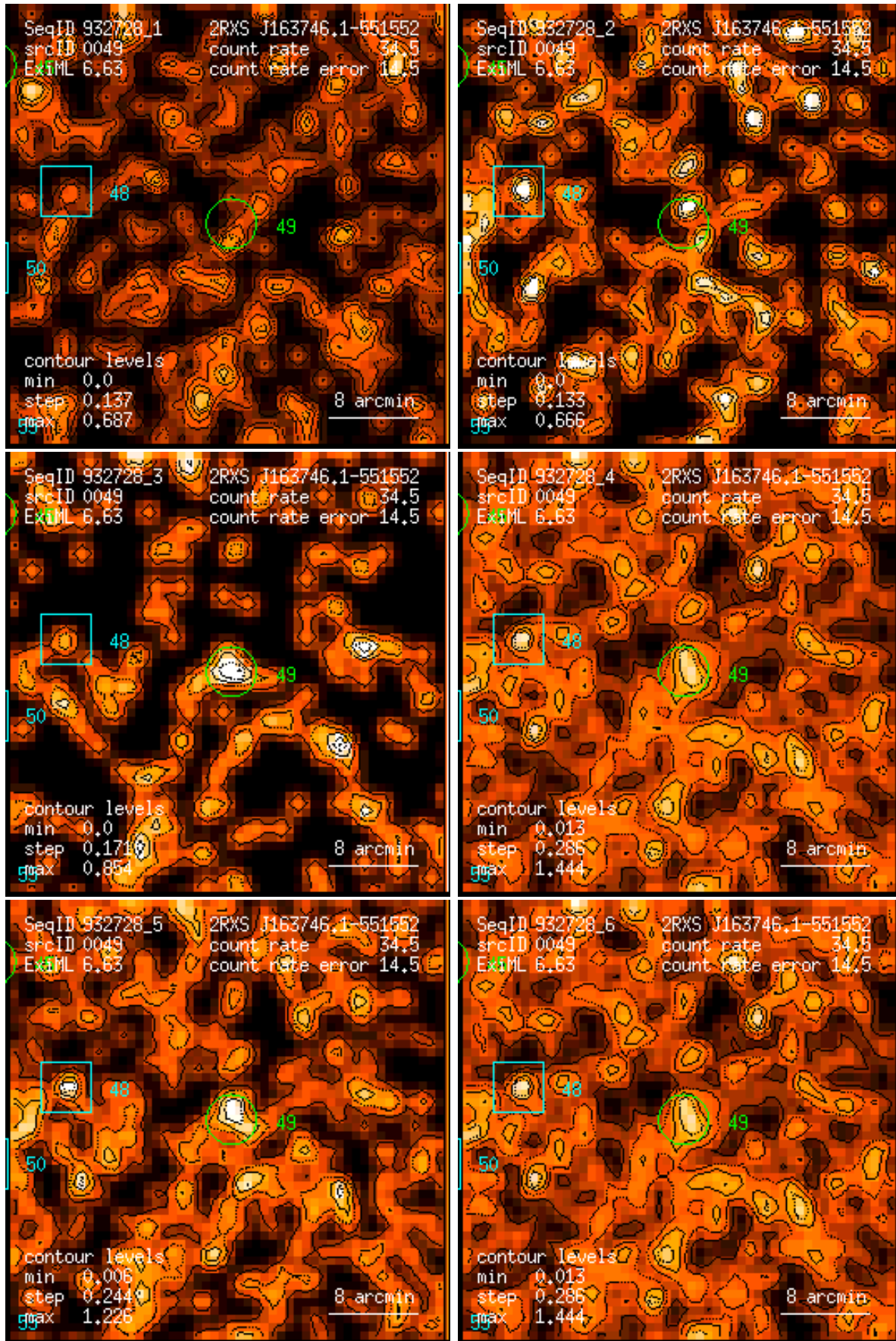
Figure 49: RASS 932728: detection 0049: band rate images, Gaussian filter: (1) PSPC channels 11 – 41, (2) 52 – 90, (3) 91 – 201, (4) 11 – 235, (5) 52 – 201, (6) 11 – 201. Broad band rates in counts/ks. Band rate contour levels in counts/ks/arcmin 2 .
