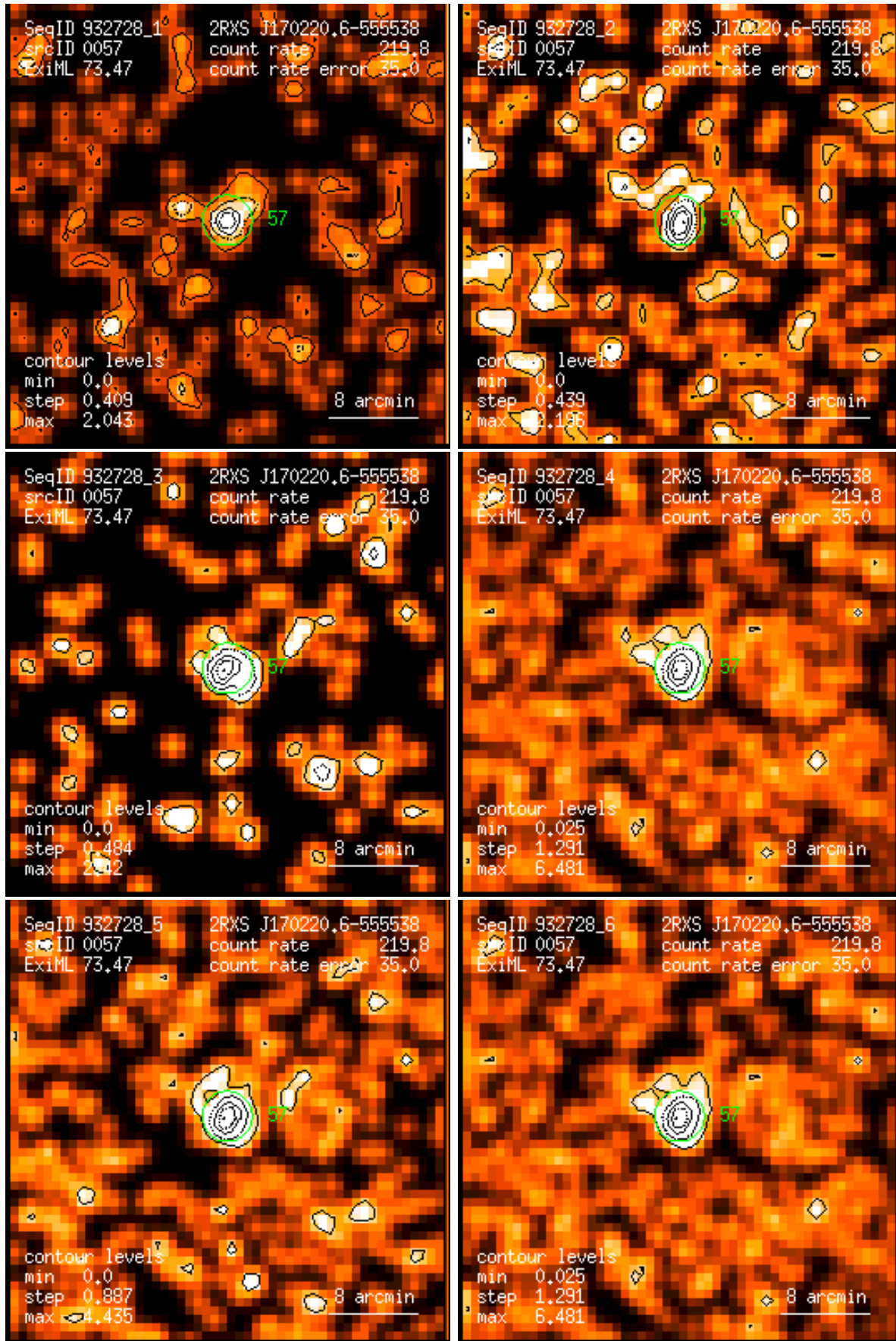
Figure 57: RASS 932728: detection 0057: band rate images, Gaussian filter: (1) PSPC channels 11 – 41, (2) 52 – 90, (3) 91 – 201, (4) 11 – 235, (5) 52 – 201, (6) 11 – 201. Broad band rates in counts/ks. Band rate contour levels in counts/ks/arcmin 2 .
