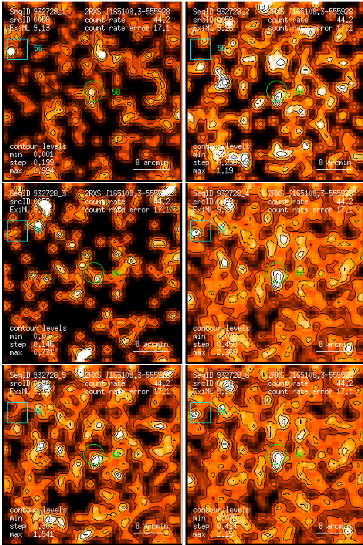
Figure 58: RASS 932728: detection 0058: band rate images, Gaussian filter: (1) PSPC channels 11 – 41, (2) 52 – 90, (3) 91 – 201, (4) 11 – 235, (5) 52 – 201, (6) 11 – 201. Broad band rates in counts/ks. Band rate contour levels in counts/ks/arcmin 2 .
