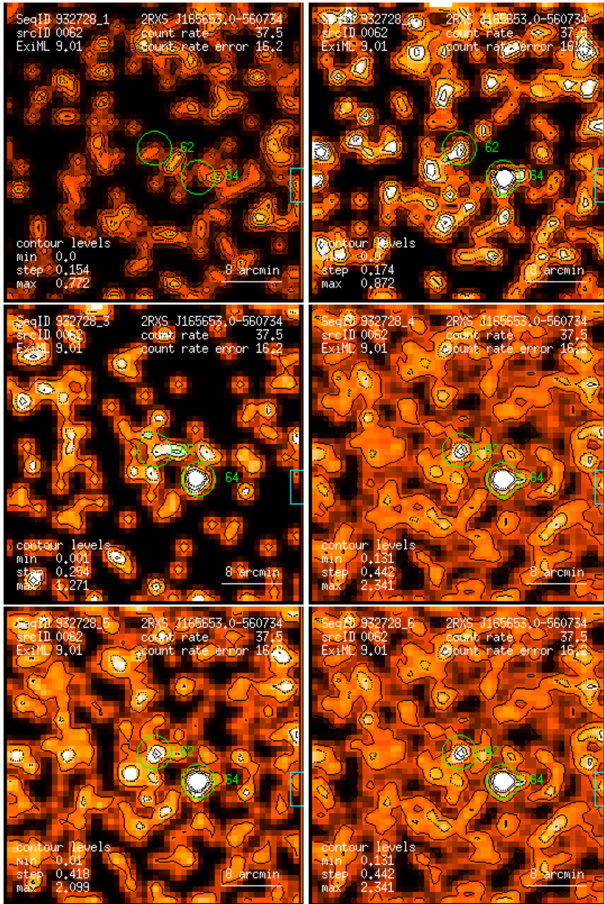
Figure 62: RASS 932728: detection 0062: band rate images, Gaussian filter: (1) PSPC channels 11 – 41, (2) 52 – 90, (3) 91 – 201, (4) 11 – 235, (5) 52 – 201, (6) 11 – 201. Broad band rates in counts/ks. Band rate contour levels in counts/ks/arcmin 2 .
