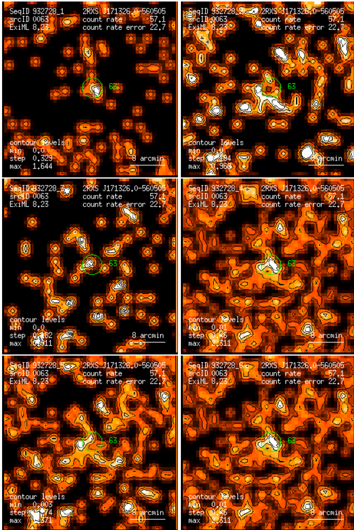
Figure 63: RASS 932728: detection 0063: band rate images, Gaussian filter: (1) PSPC channels 11 – 41, (2) 52 – 90, (3) 91 – 201, (4) 11 – 235, (5) 52 – 201, (6) 11 – 201. Broad band rates in counts/ks. Band rate contour levels in counts/ks/arcmin 2 .
