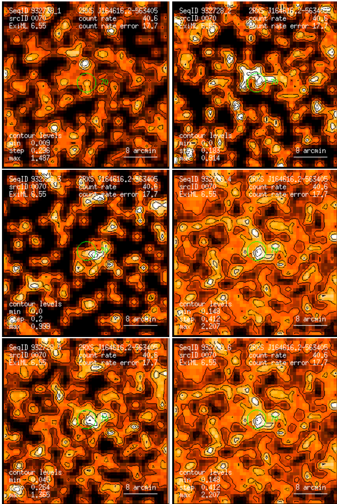
Figure 70: RASS 932728: detection 0070: band rate images, Gaussian filter: (1) PSPC channels 11 – 41, (2) 52 – 90, (3) 91 – 201, (4) 11 – 235, (5) 52 – 201, (6) 11 – 201. Broad band rates in counts/ks. Band rate contour levels in counts/ks/arcmin 2 .
